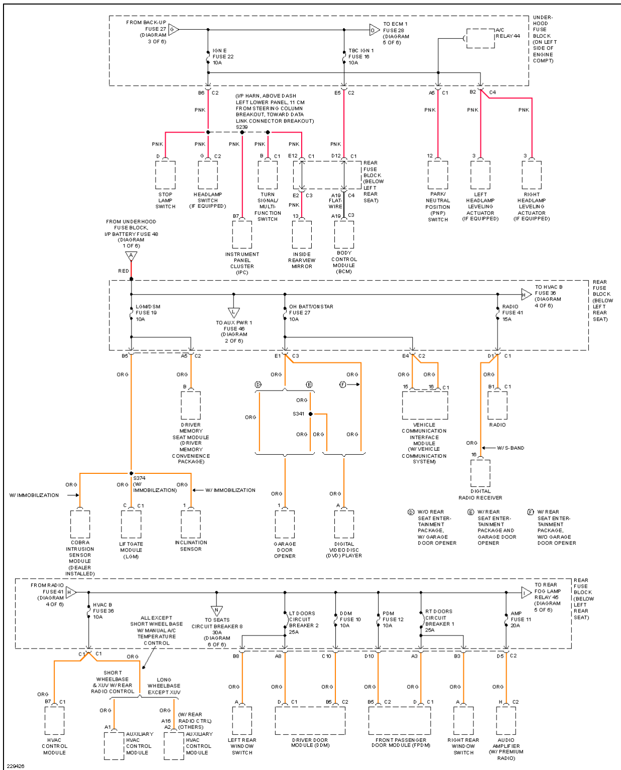
Fig. 64: Power Distribution Circuit (4 of 6)
