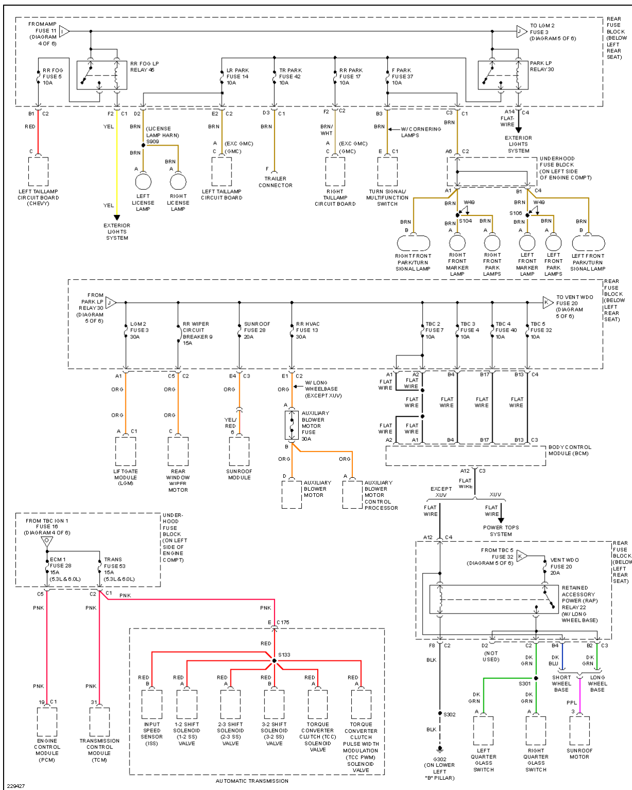
Fig. 65: Power Distribution Circuit (5 of 6)
