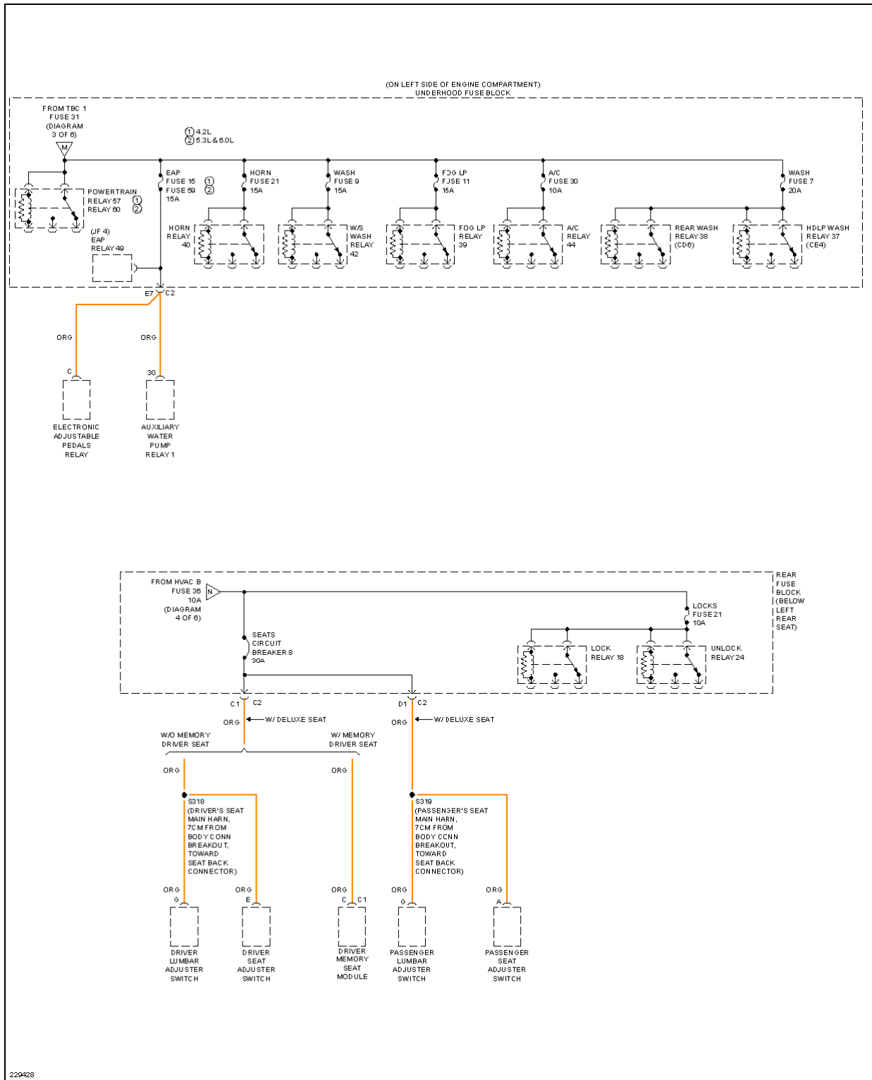
Fig. 66: Power Distribution Circuit (6 of 6)
