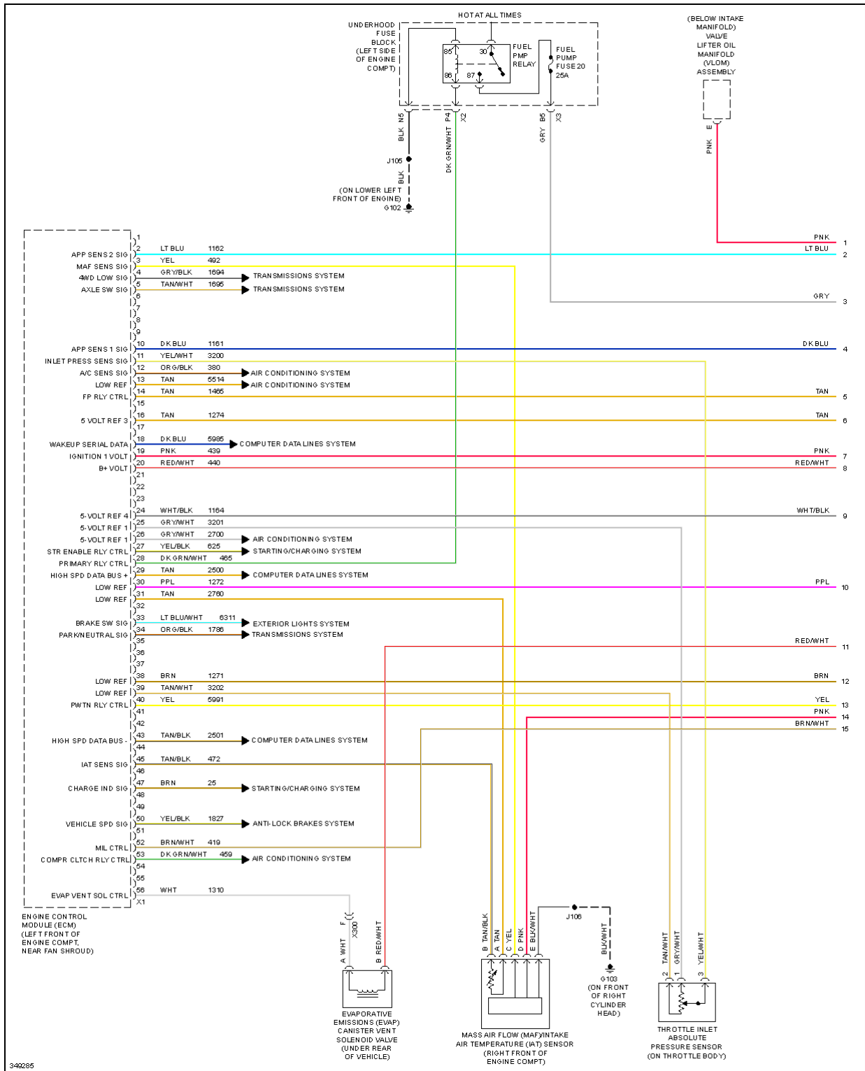
Fig. 27: 6.0L VIN G, Engine Performance Circuit (1 of 6)
