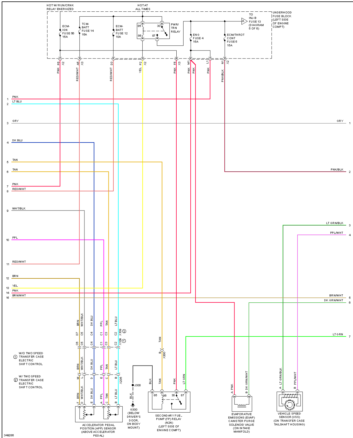
Fig. 28: 6.0L VIN G, Engine Performance Circuit (2 of 6)
