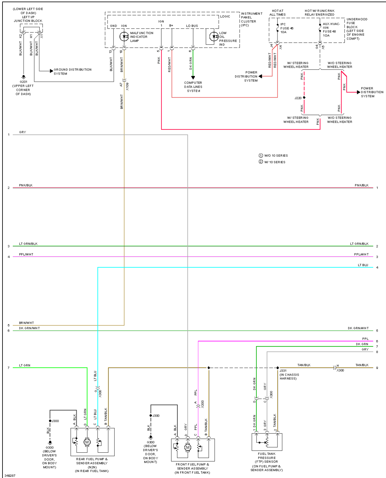
Fig. 29: 6.0L VIN G, Engine Performance Circuit (3 of 6)
