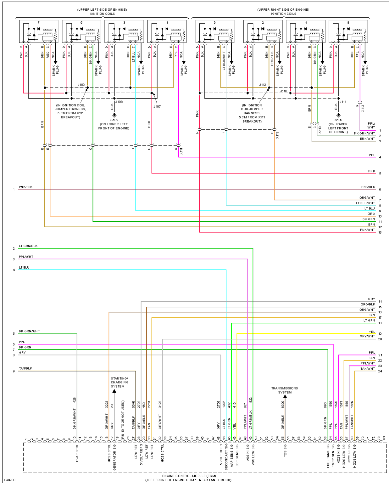
Fig. 30: 6.0L VIN G, Engine Performance Circuit (4 of 6)
