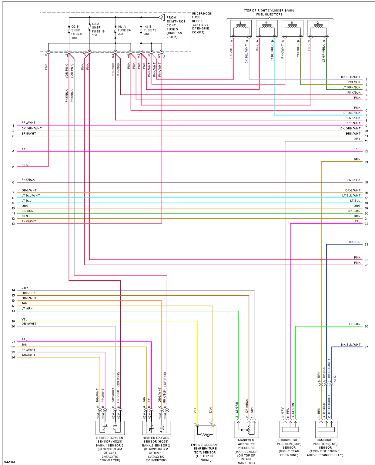
Fig. 31: 6.0L VIN G, Engine Performance Circuit (5 of 6)
