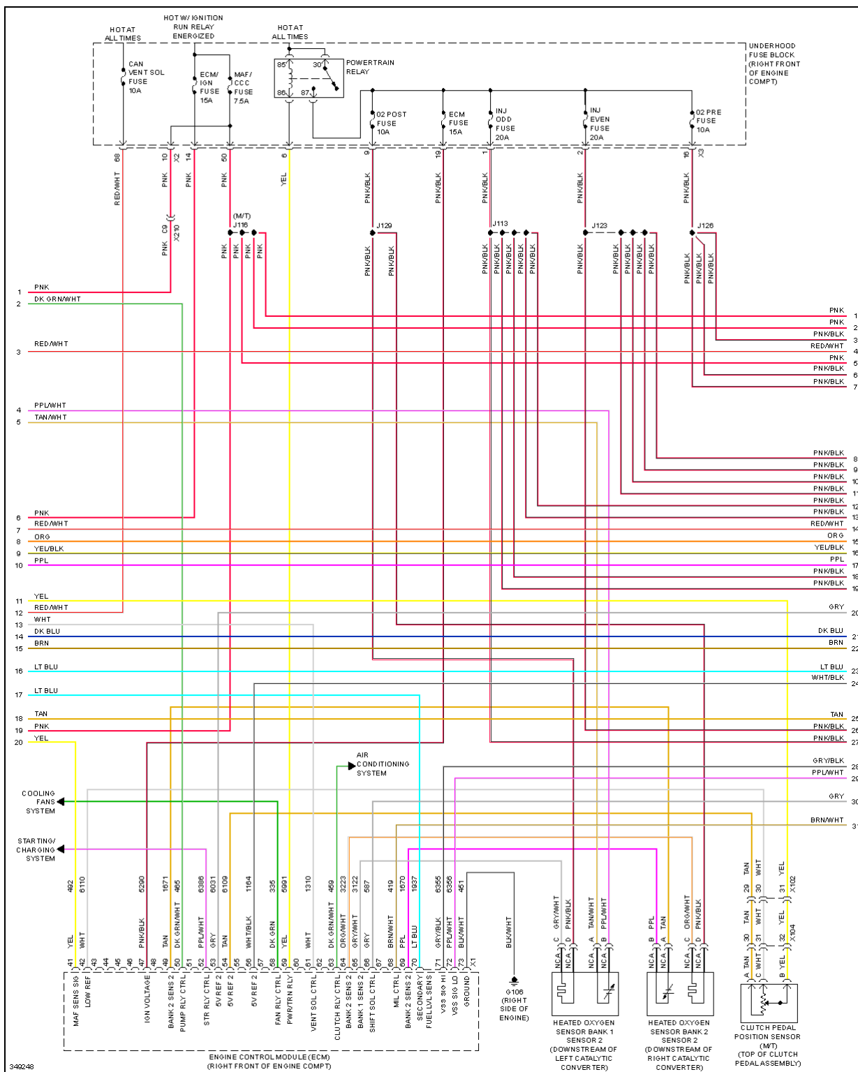
Fig. 27: 6.2L VIN W, Engine Performance Circuit (2 of 6)
