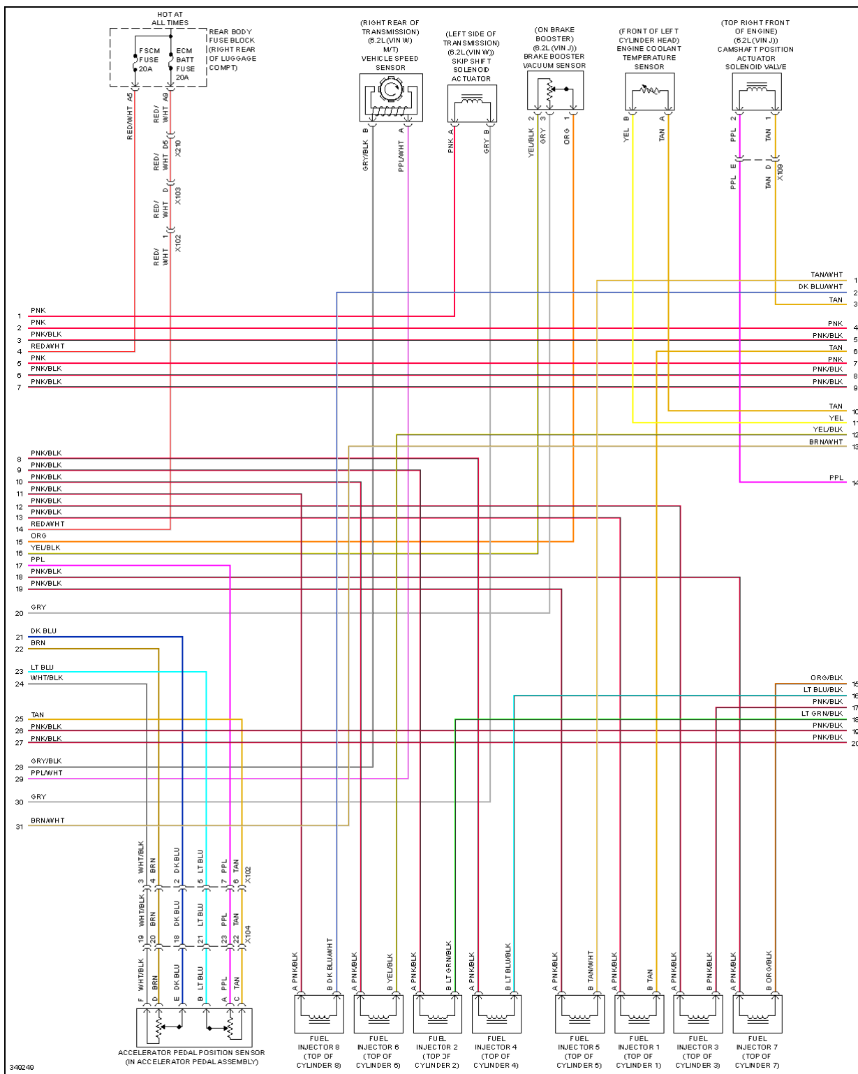
Fig. 28: 6.2L VIN W, Engine Performance Circuit (3 of 6)
