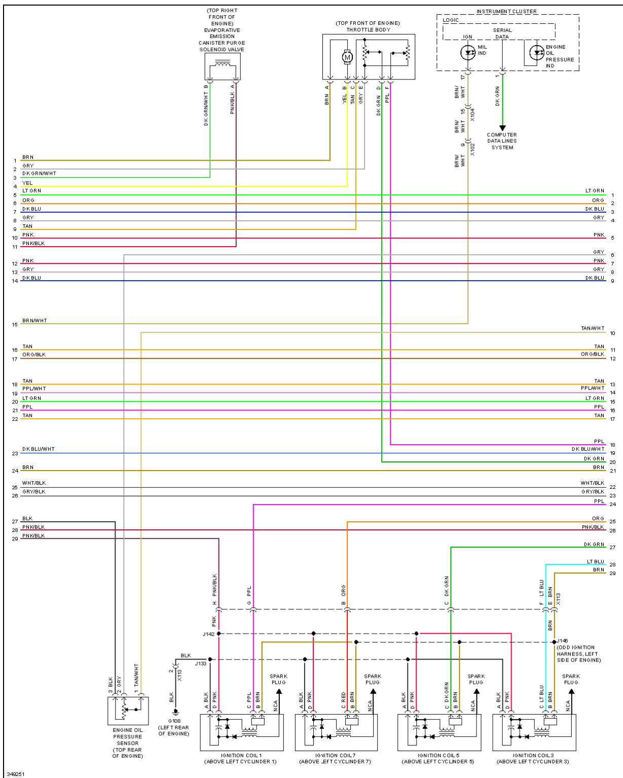
Fig. 30: 6.2L VIN W, Engine Performance Circuit (5 of 6)
