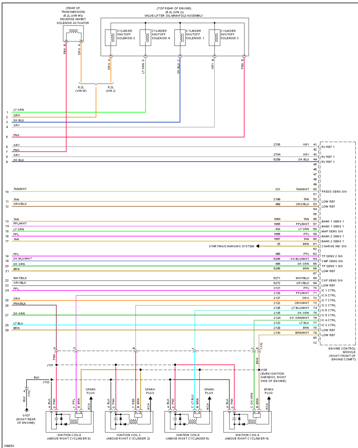
Fig. 31: 6.2L VIN W, Engine Performance Circuit (6 of 6)
