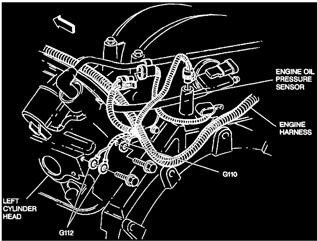
Upper Left Rear Side Of Engine
