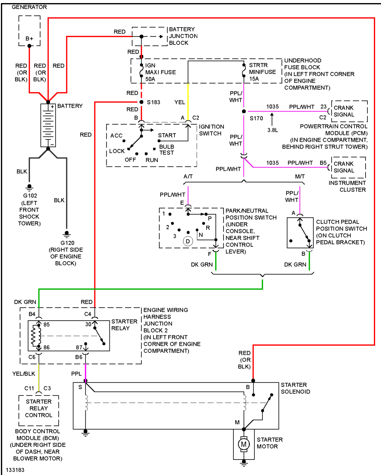
Fig. 50: Starting Circuit
