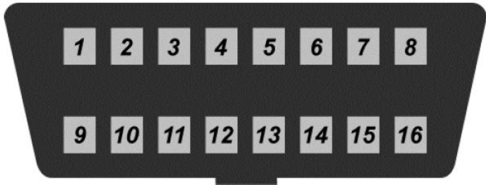
Vehicle OBDII Socket SAE J1962 Female
