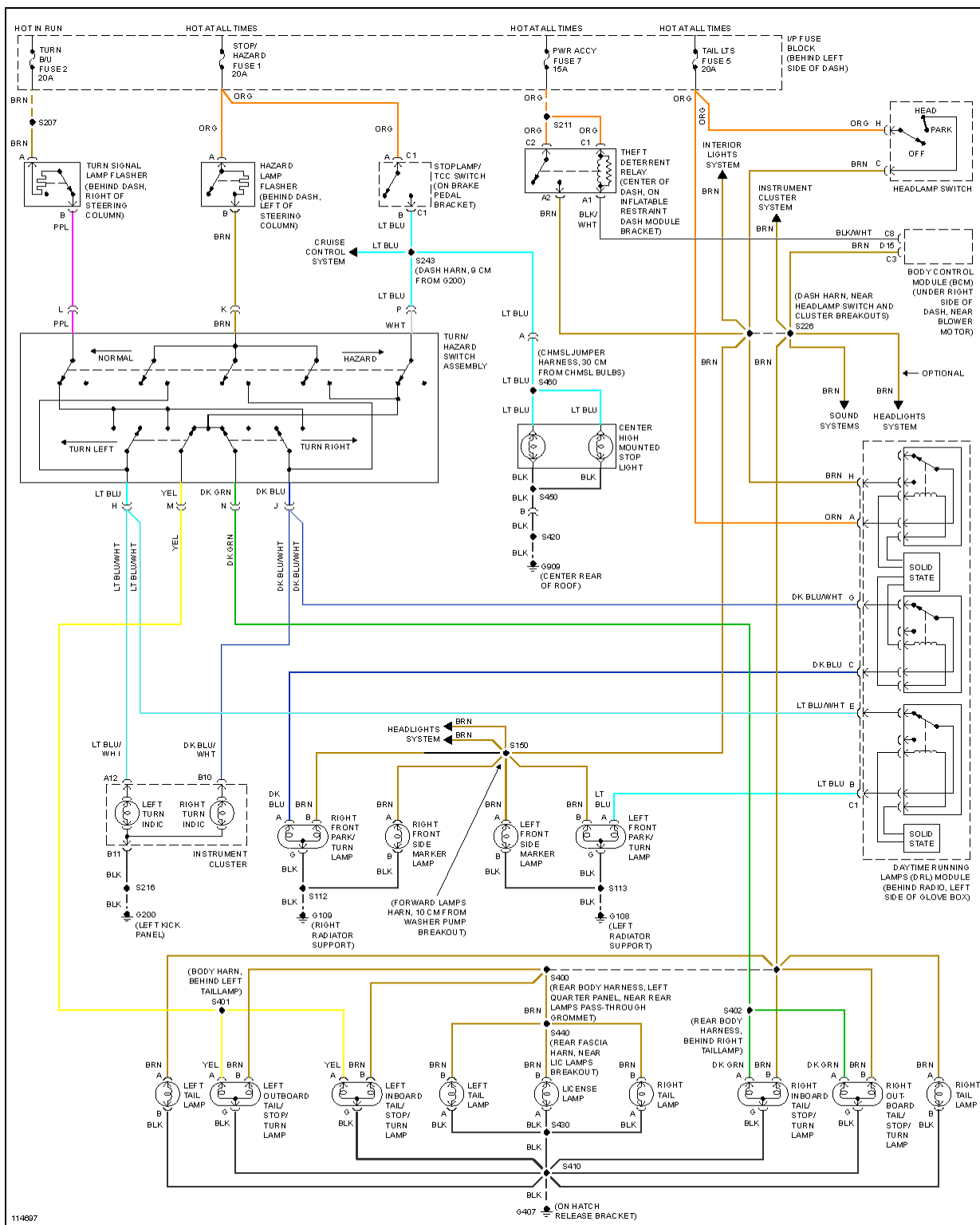
Fig. 25: Exterior Lamps Circuit
