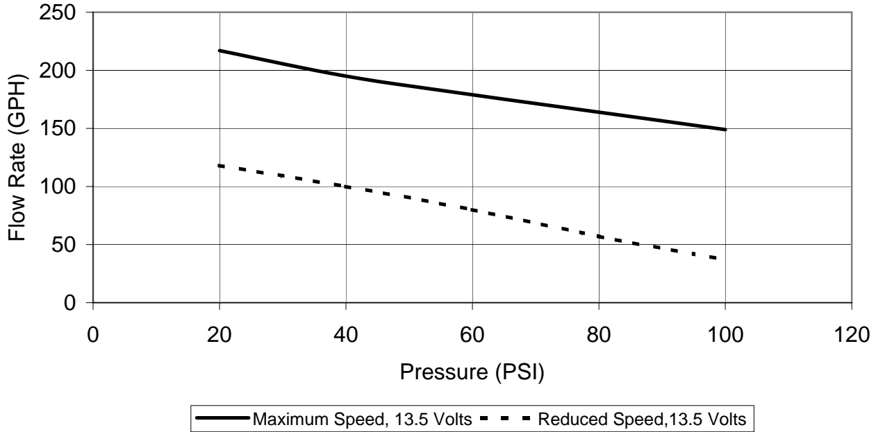
Flow Performance Graph
