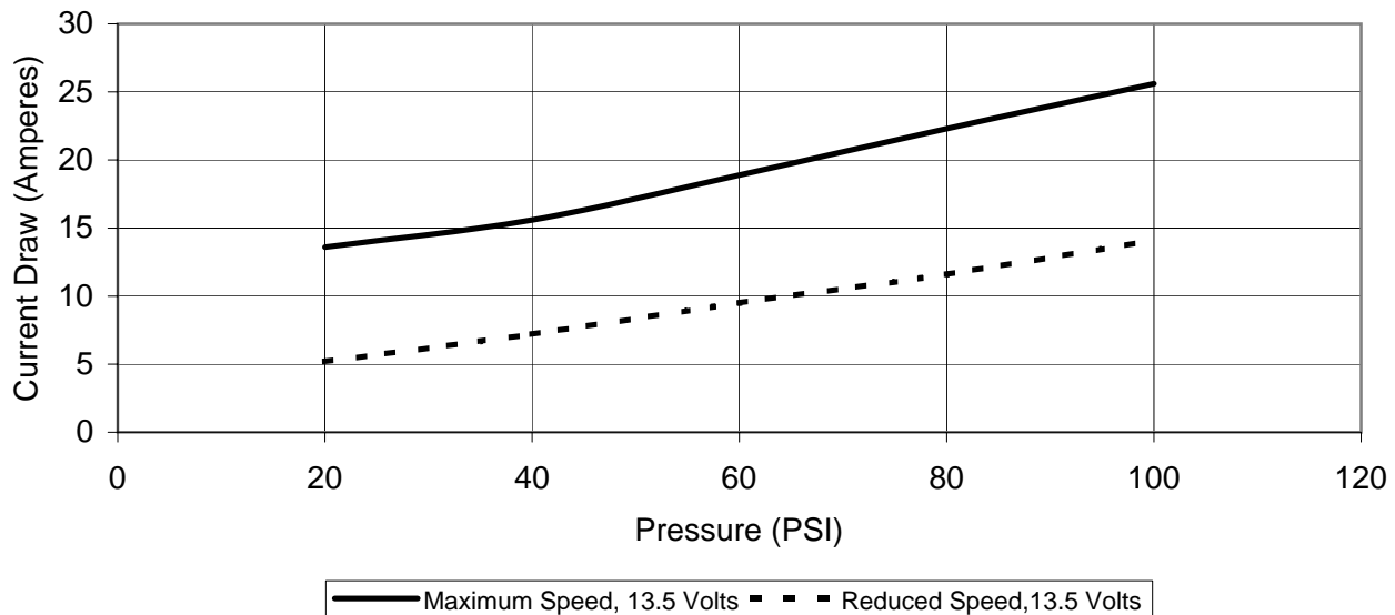
Current Draw Graph
