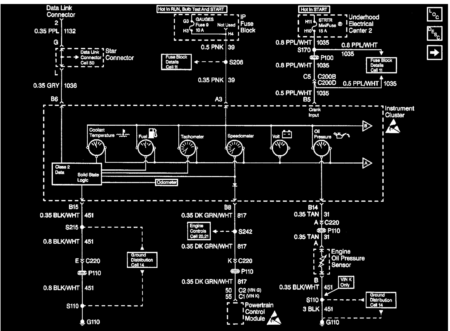
Instrument Cluster Analog Schematics: Data Link, Engine Oil Pressure Sensor, Instrument Cluster, And PCM
