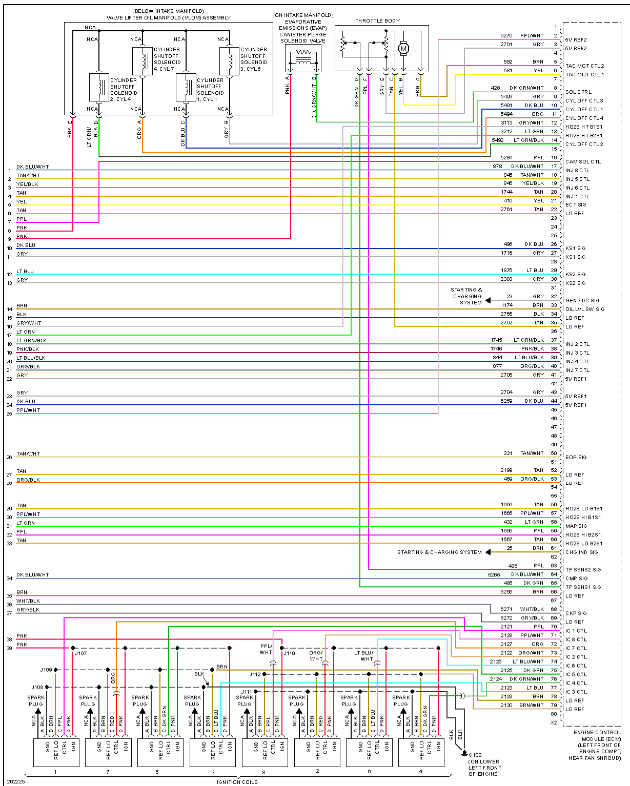
Fig. 40: 5.3L VIN 0, Engine Performance Circuit (4 of 4)
