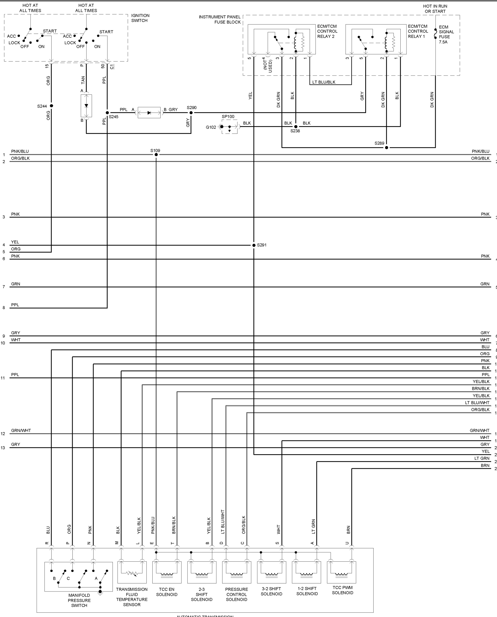
AUTOMATIC TRANSMISSION
