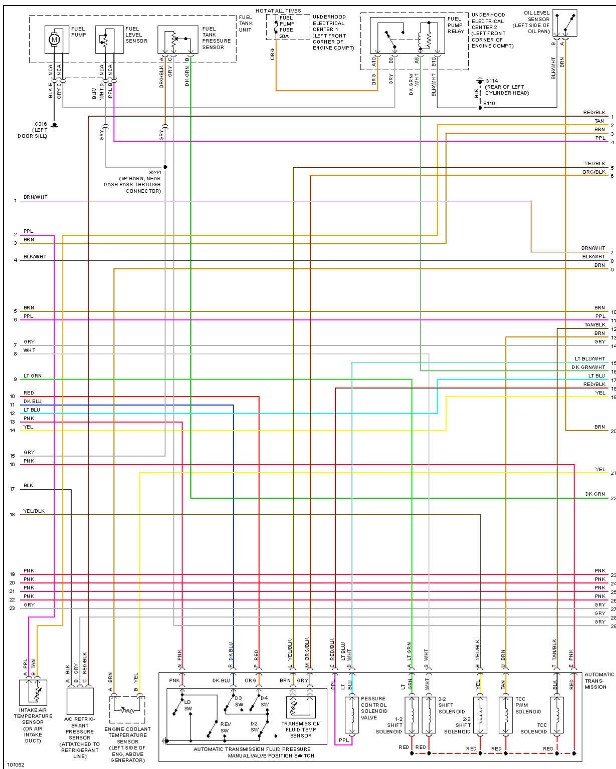
Fig. 17: 5.7L (VIN G), Engine Performance Circuits (3 of 4)
