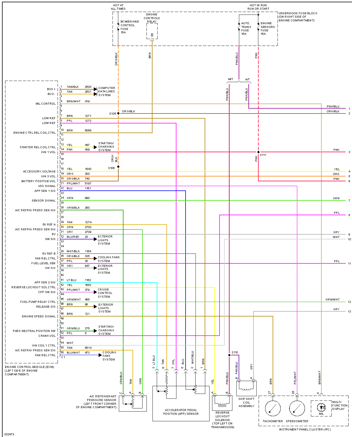
Fig. 11: 6.0L VIN U, Engine Performance Circuit (1 of 6)
