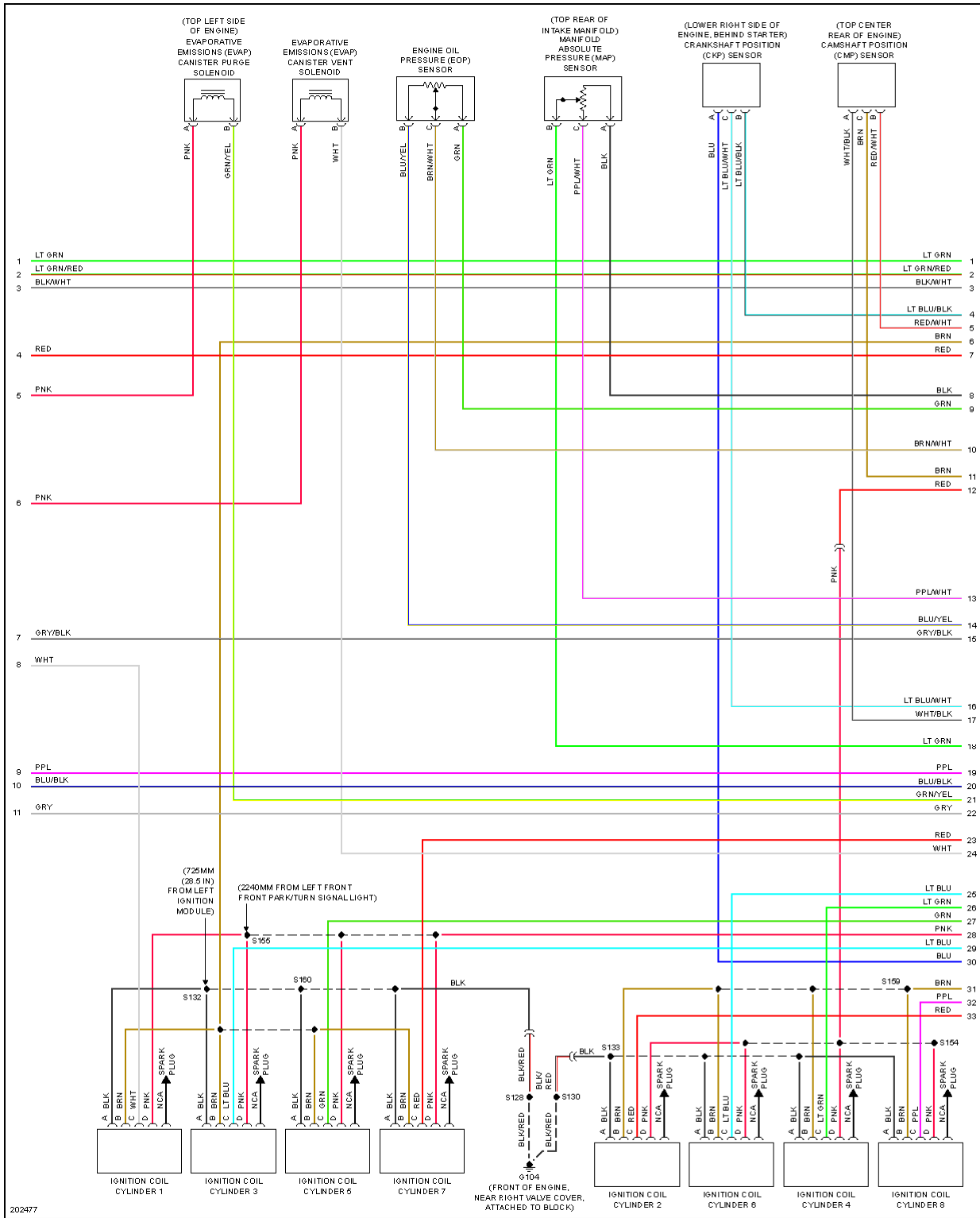
Fig. 15: 6.0L VIN U, Engine Performance Circuit (5 of 6)
