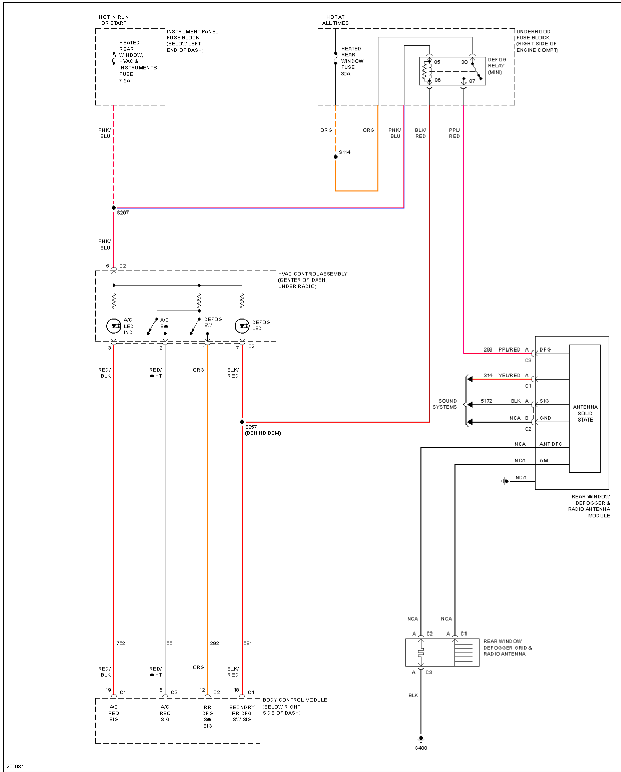
Fig. 10: Defoggers Circuit
