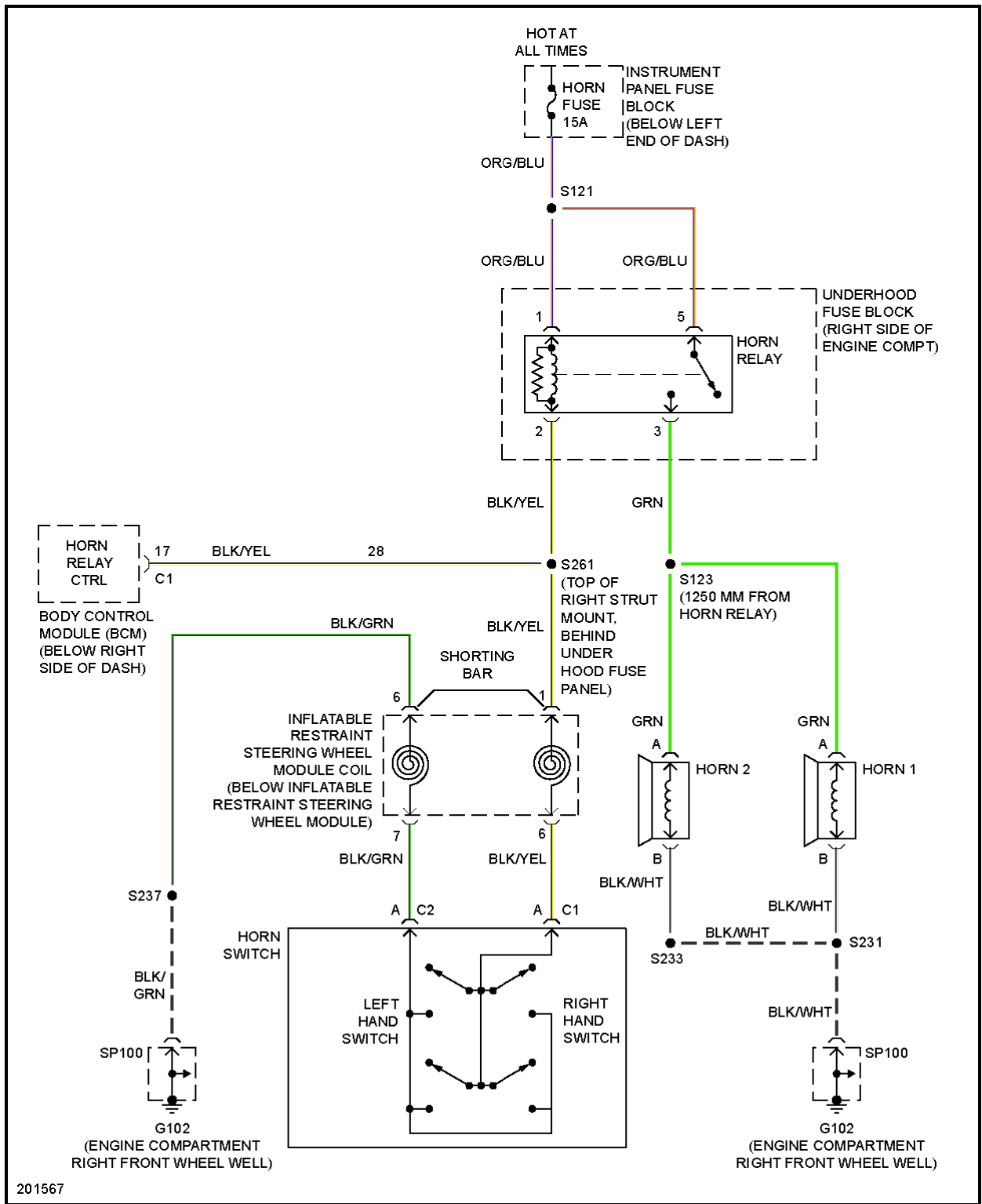
Fig. 25: Horn Circuit
