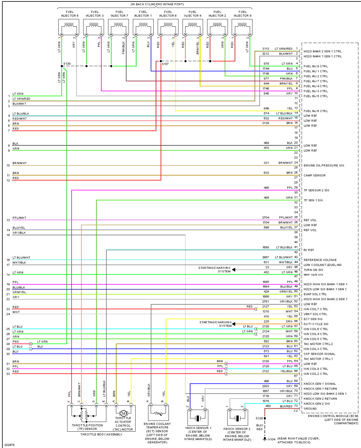
Fig. 16: 6.0L VIN U, Engine Performance Circuit (6 of 6)
