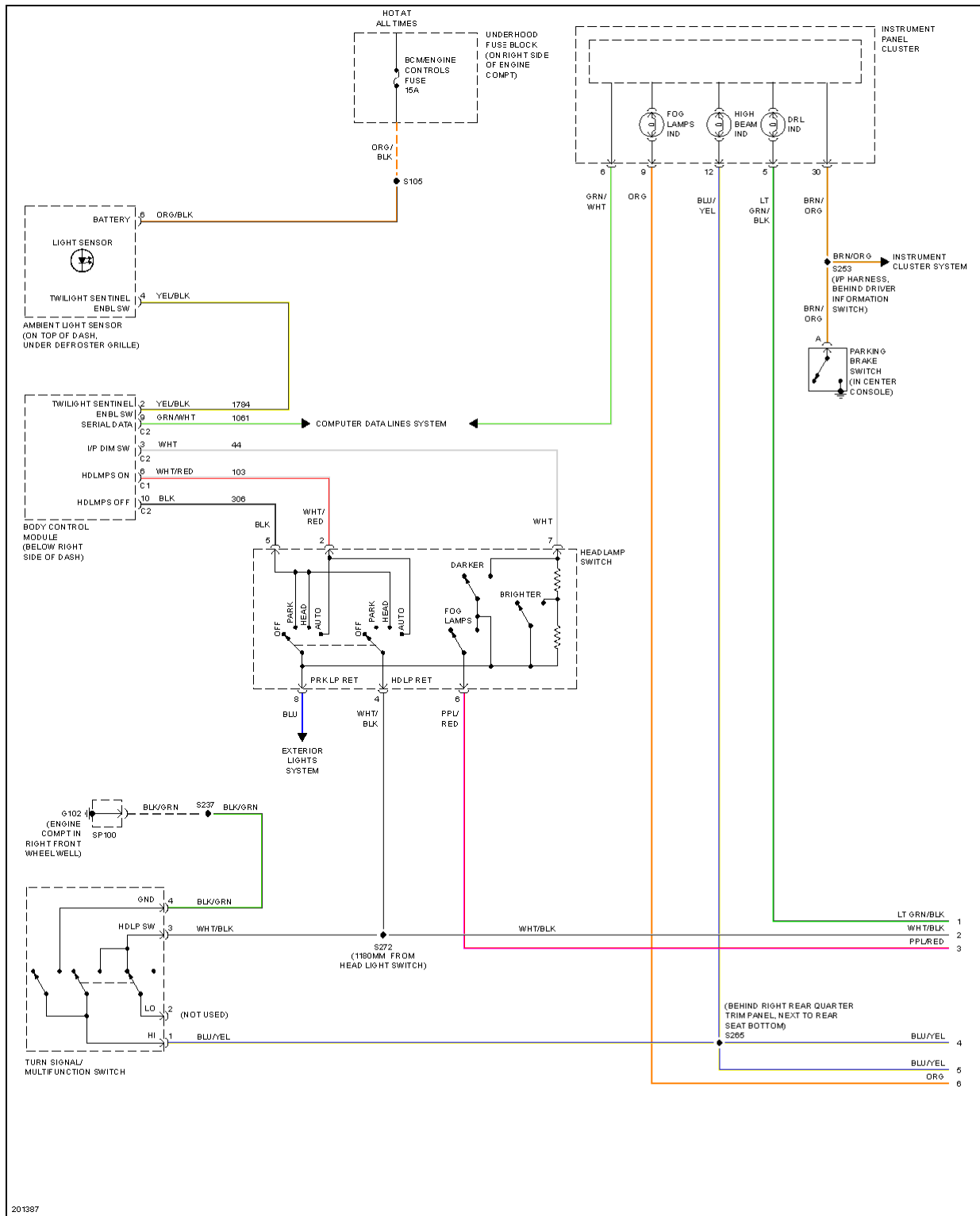
Fig. 23: Headlights Circuit (1 of 2)
