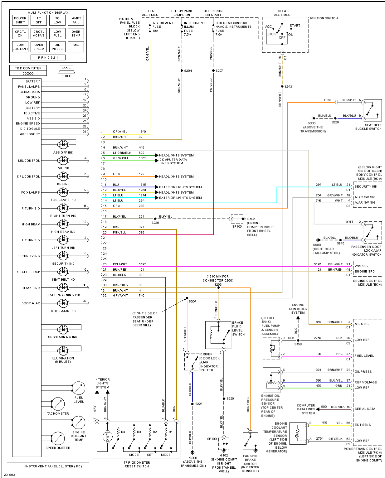
Fig. 26: Instrument Cluster Circuit
