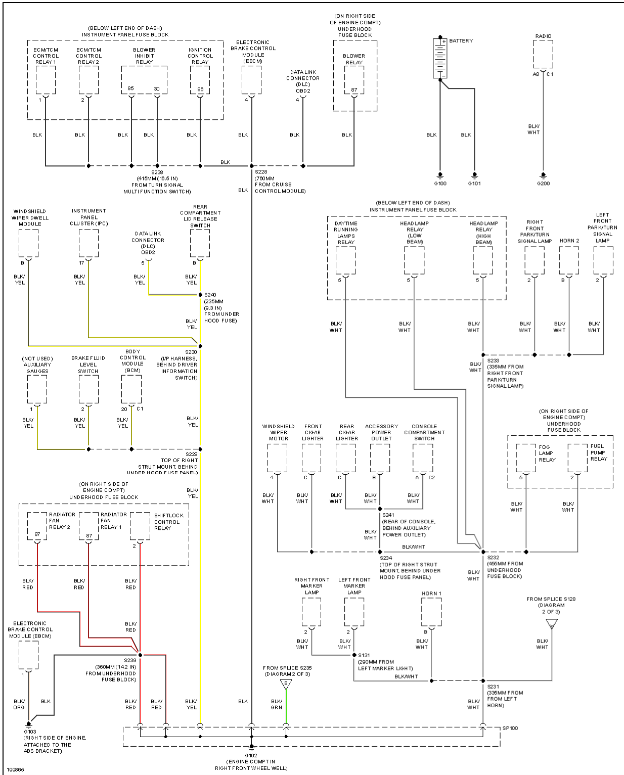
Fig. 20: Ground Distribution Circuit (1 of 3)
