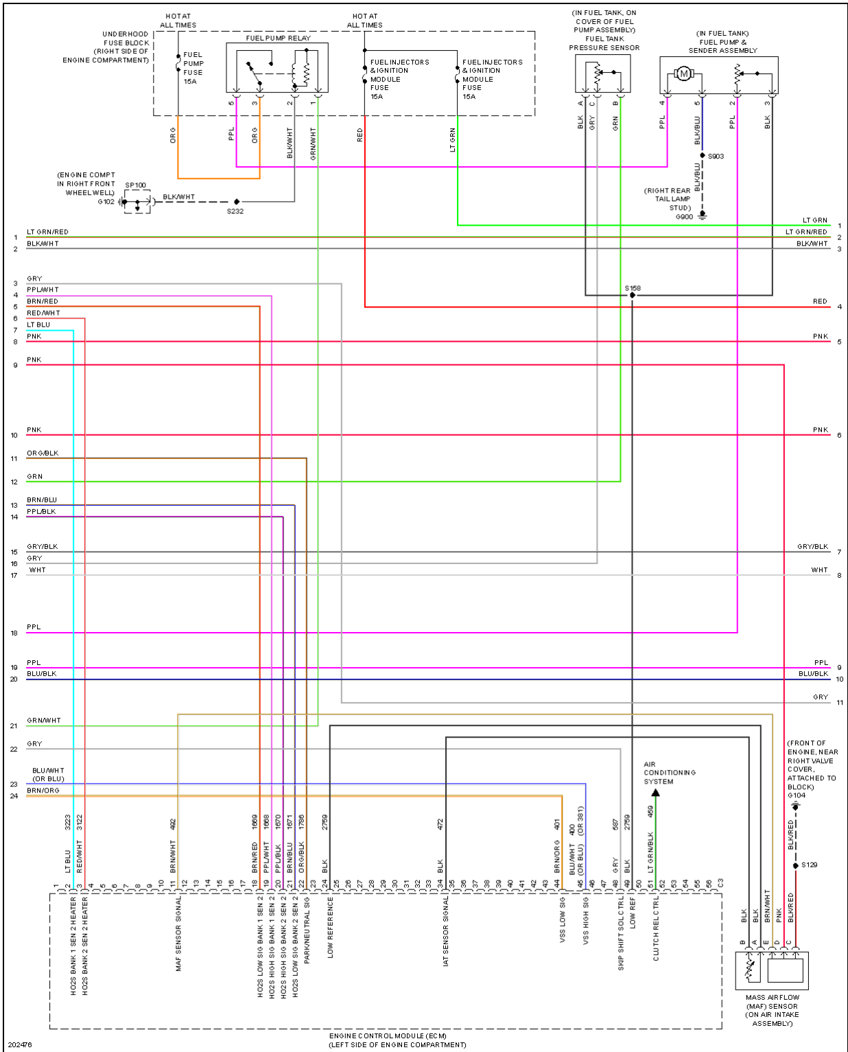
Fig. 14: 6.0L VIN U, Engine Performance Circuit (4 of 6)
