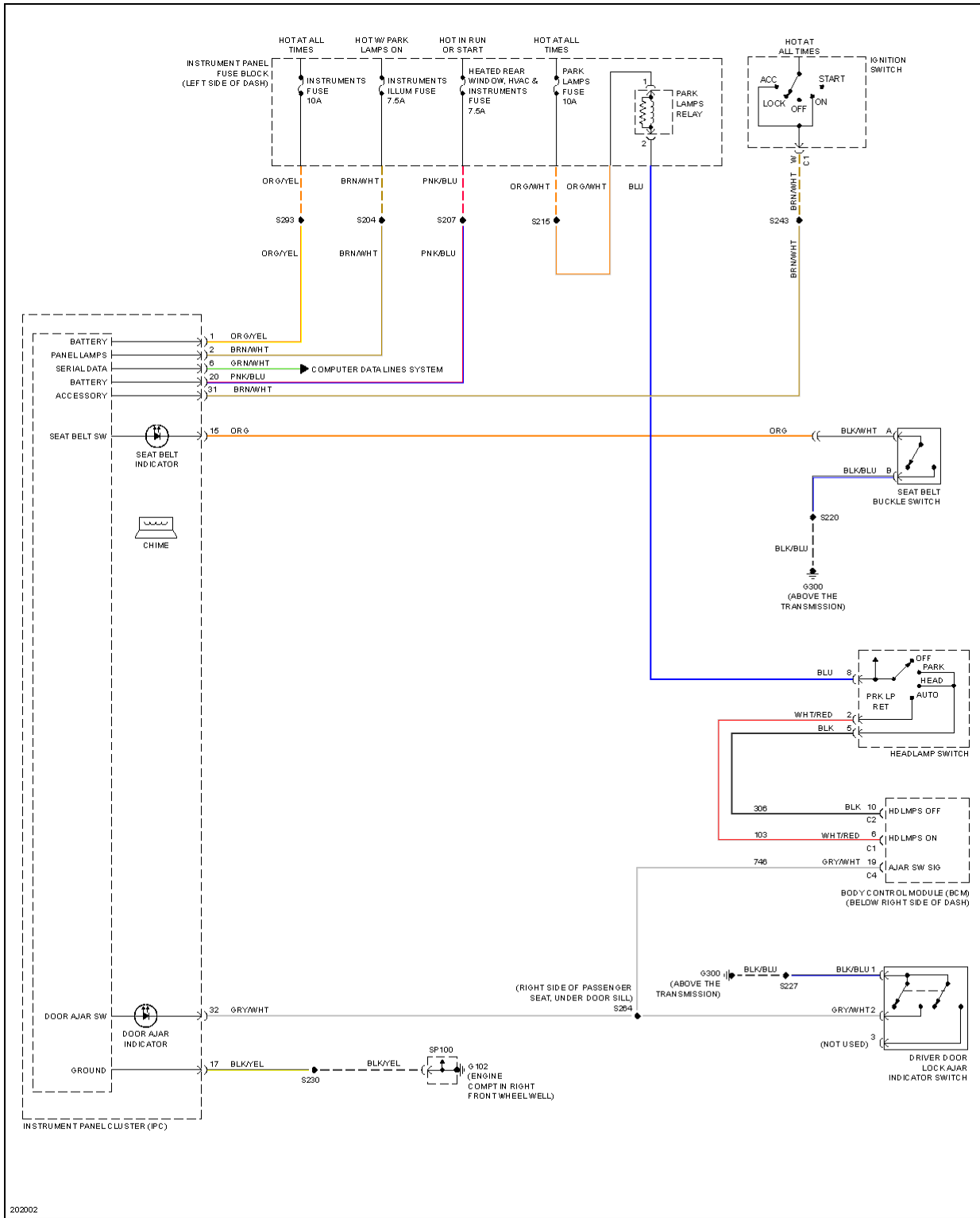
Fig. 46: Warning Systems Circuit
