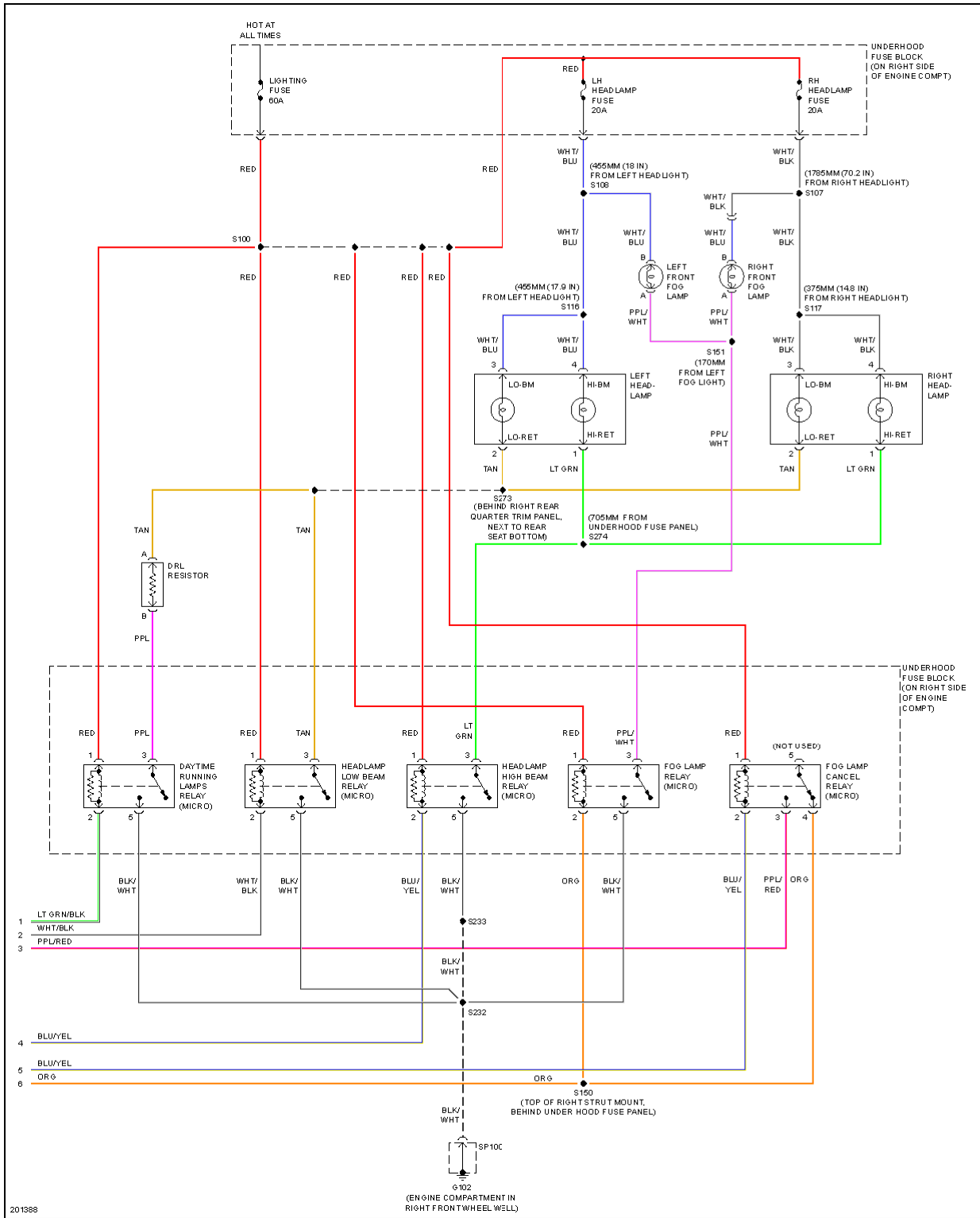
Fig. 24: Headlights Circuit (2 of 2)
