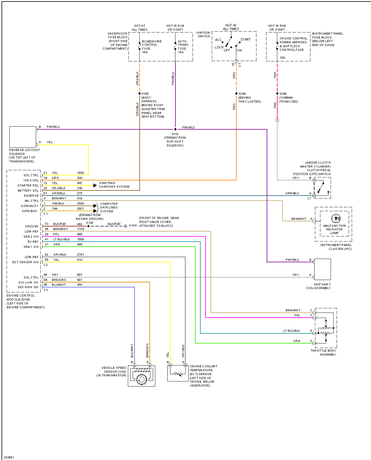
Fig. 44: M/T Circuit
