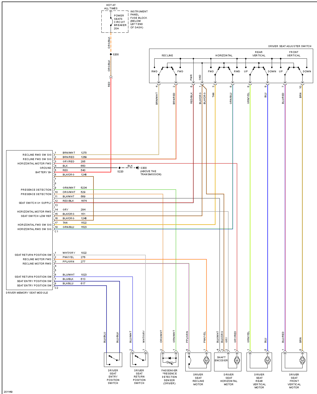
Fig. 34: Driver Power Seat Circuit
