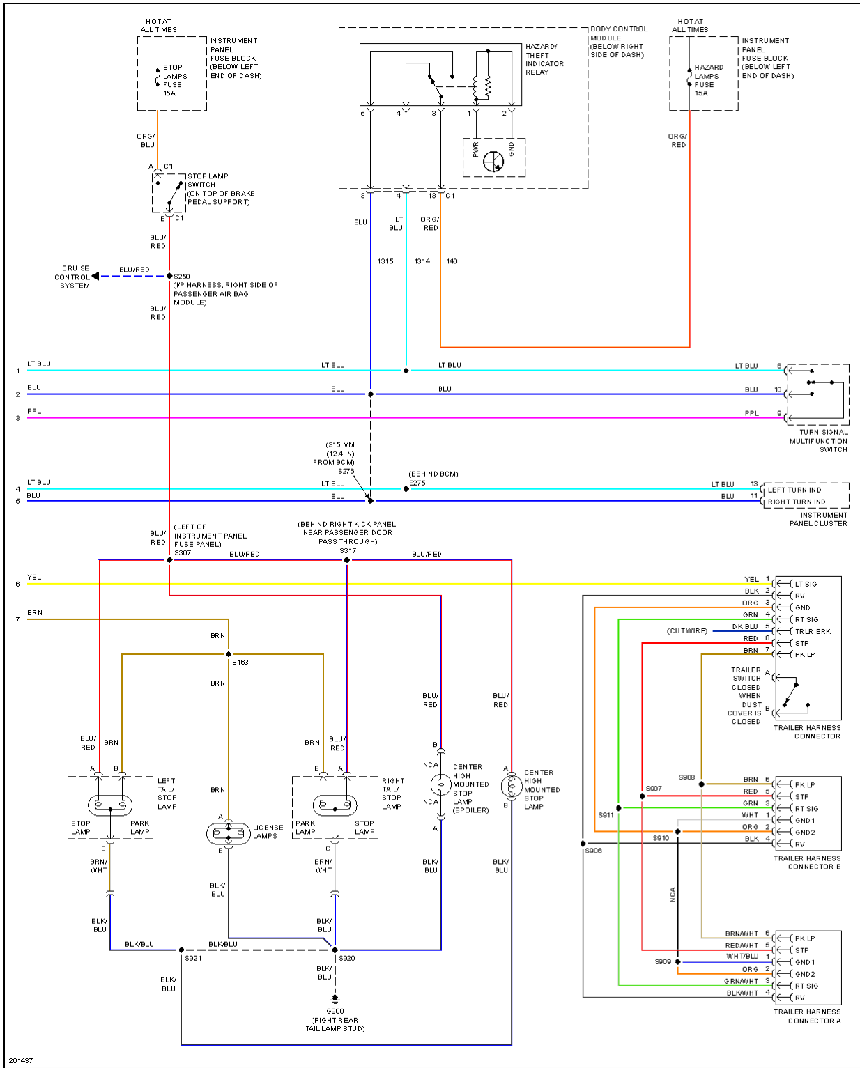
Fig. 19: Exterior Lamps Circuit (2 of 2)
