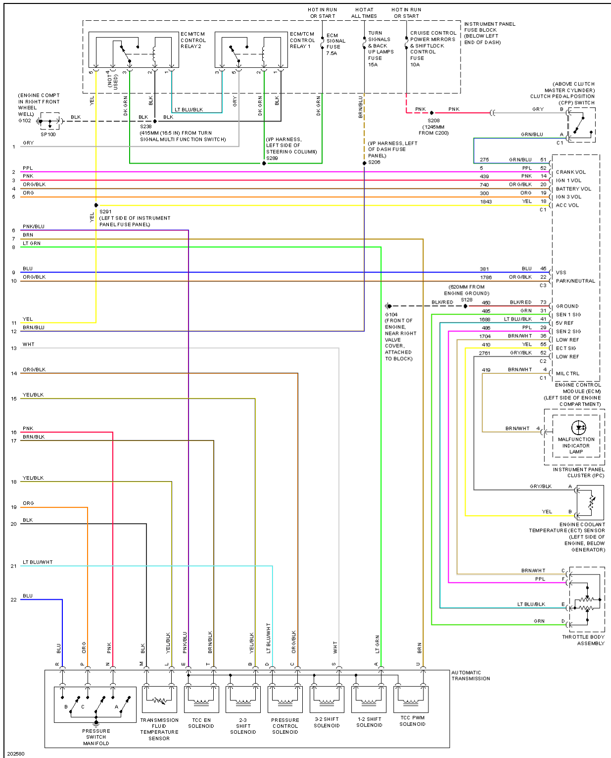
Fig. 43: A/T Circuit (2 of 2)
