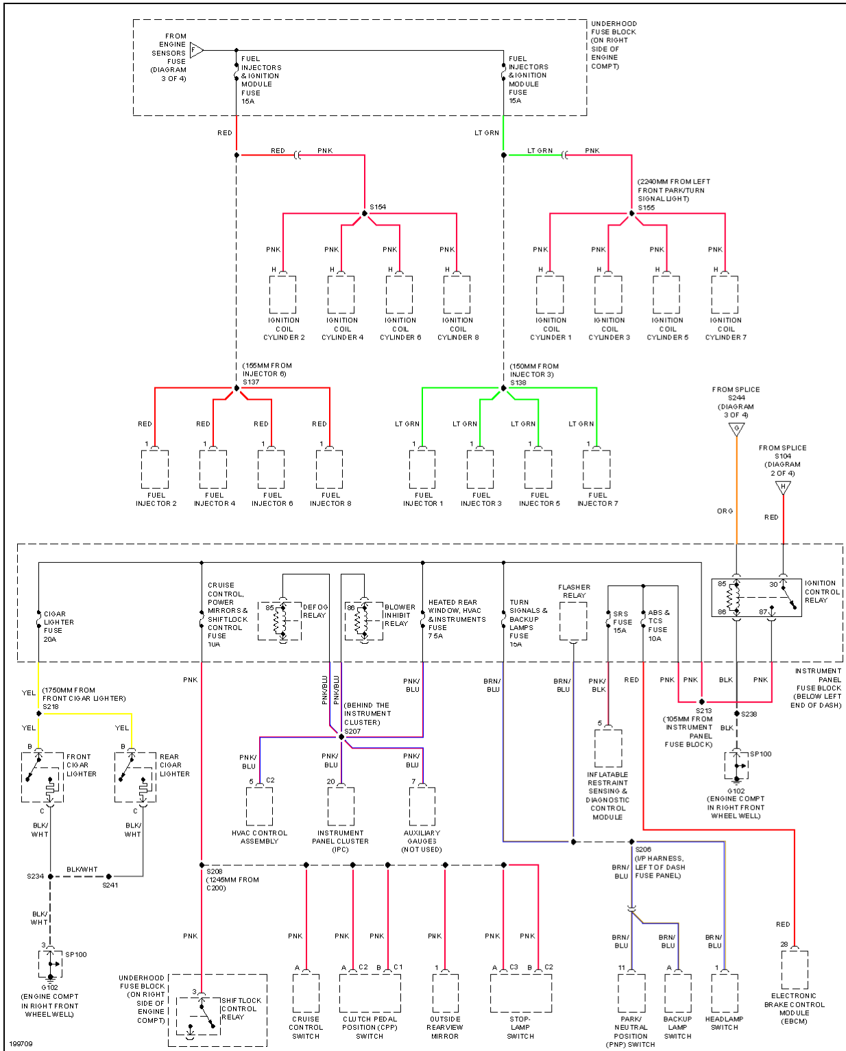
Fig. 32: Power Distribution Circuit (4 of 4)
