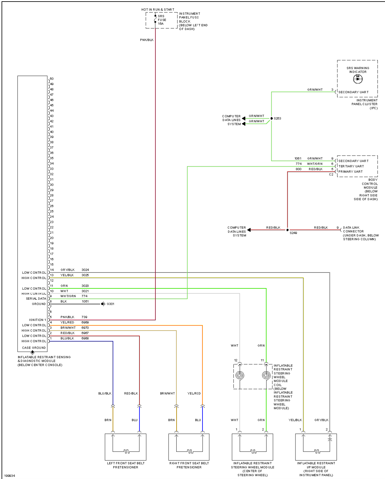
Fig. 41: Supplemental Restraints Circuit
