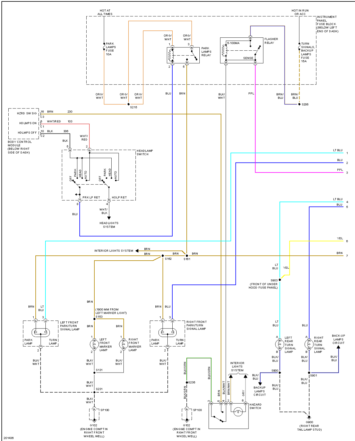
Fig. 18: Exterior Lamps Circuit (1 of 2)
