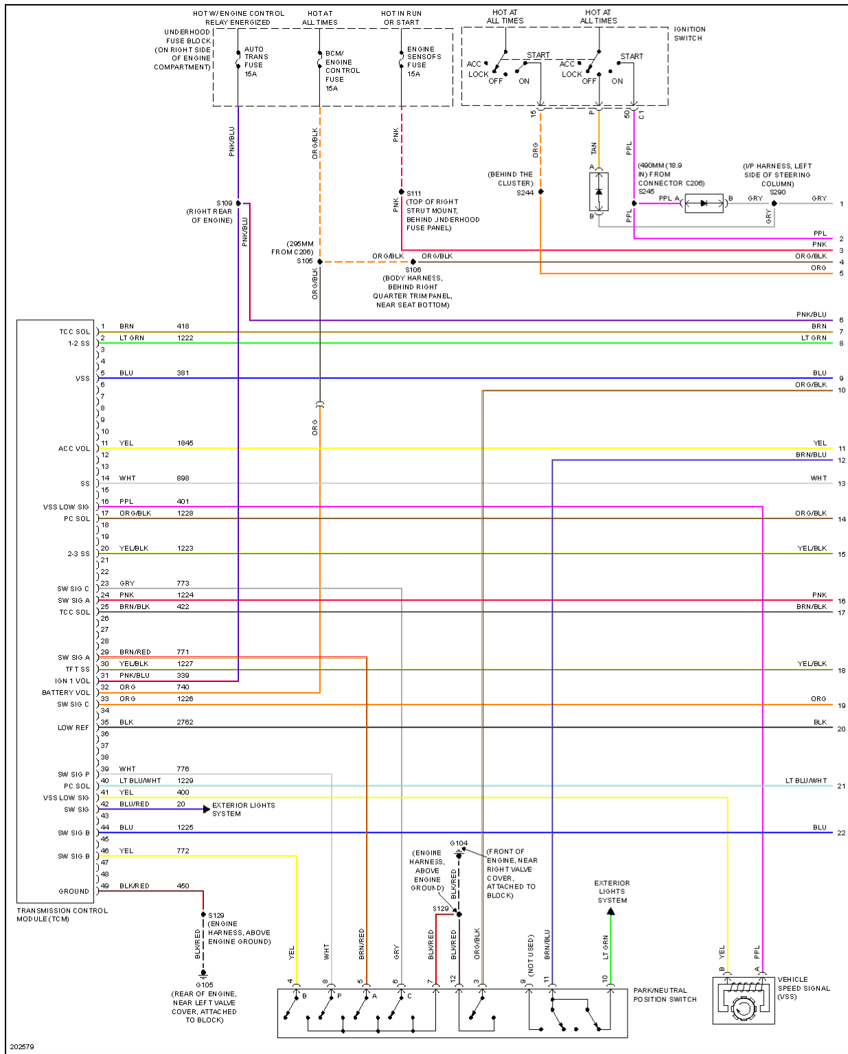
Fig. 42: A/T Circuit (1 of 2)
