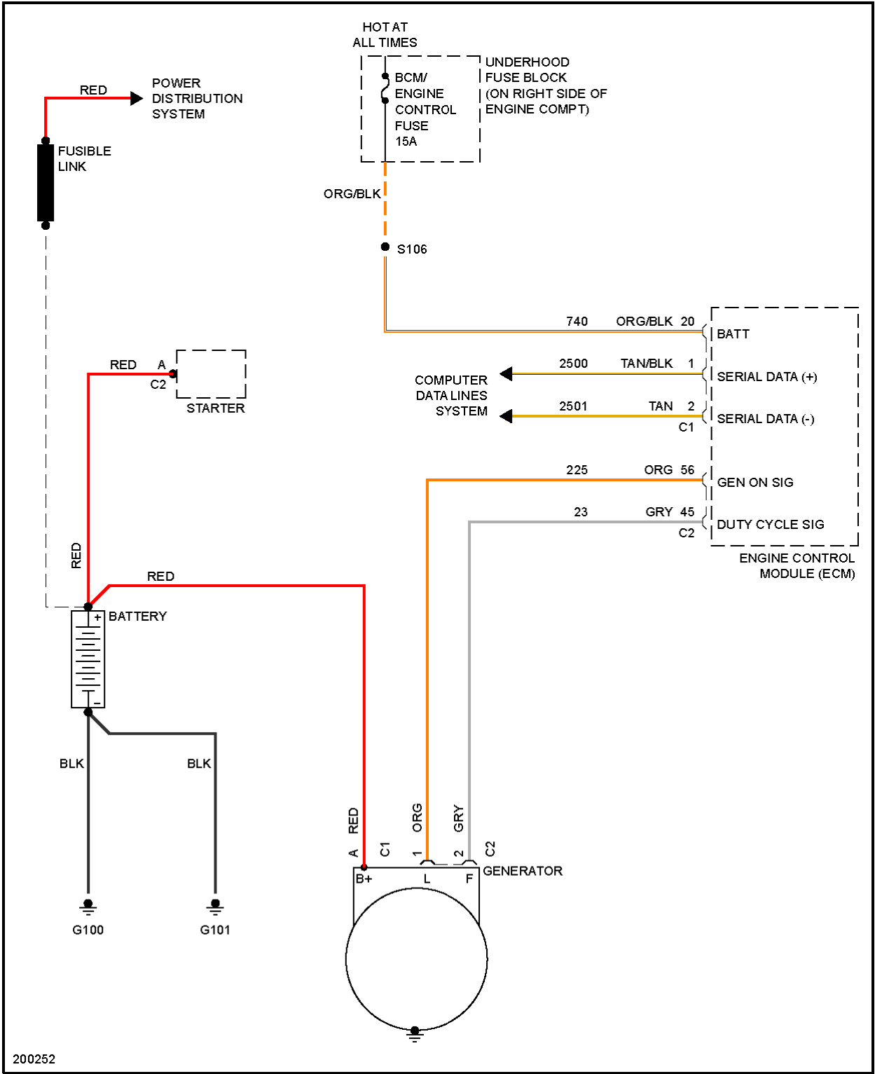
Fig. 39: Charging Circuit
