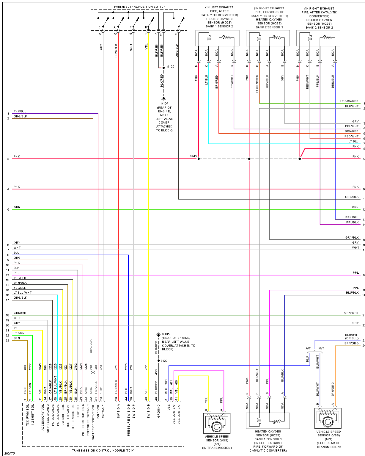
Fig. 13: 6.0L VIN U, Engine Performance Circuit (3 of 6)
