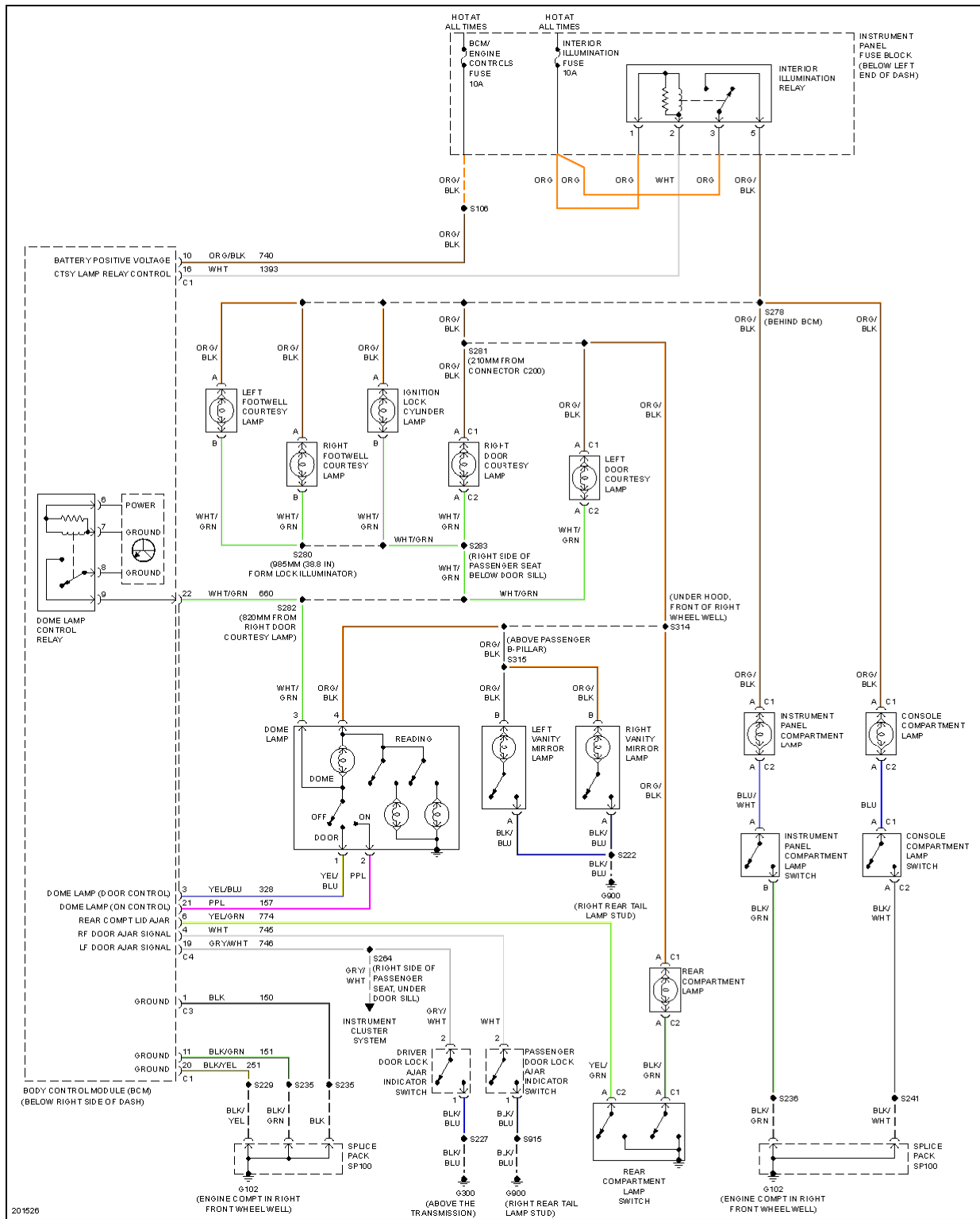
Fig. 27: Courtesy Lamps Circuit
