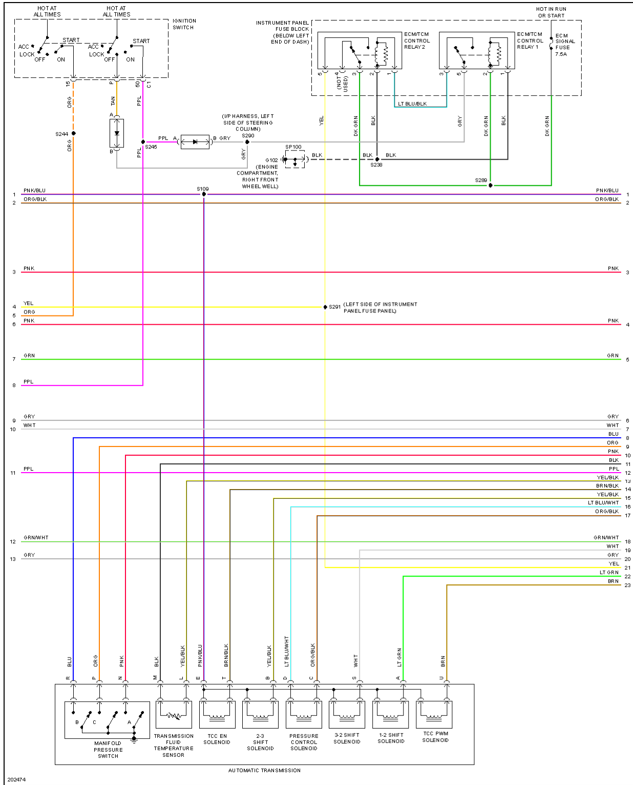
Fig. 12: 6.0L VIN U, Engine Performance Circuit (2 of 6)
