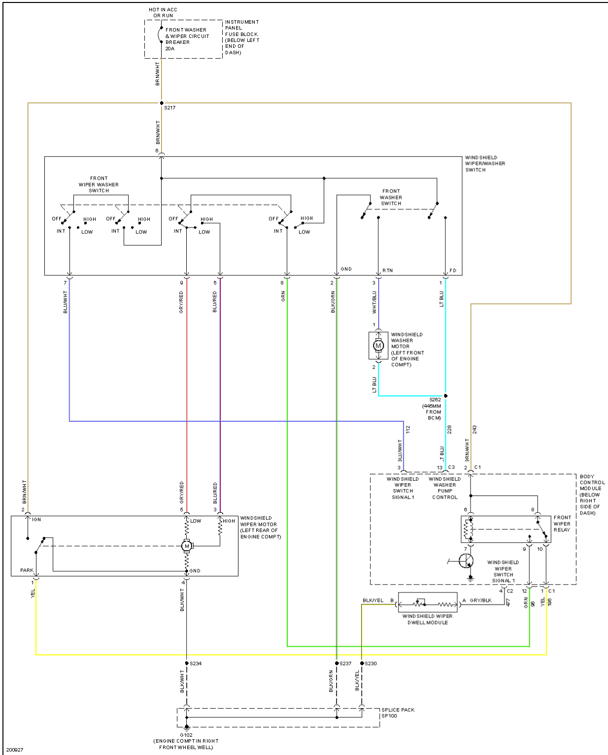
Fig. 47: Wiper/Washer Circuit
