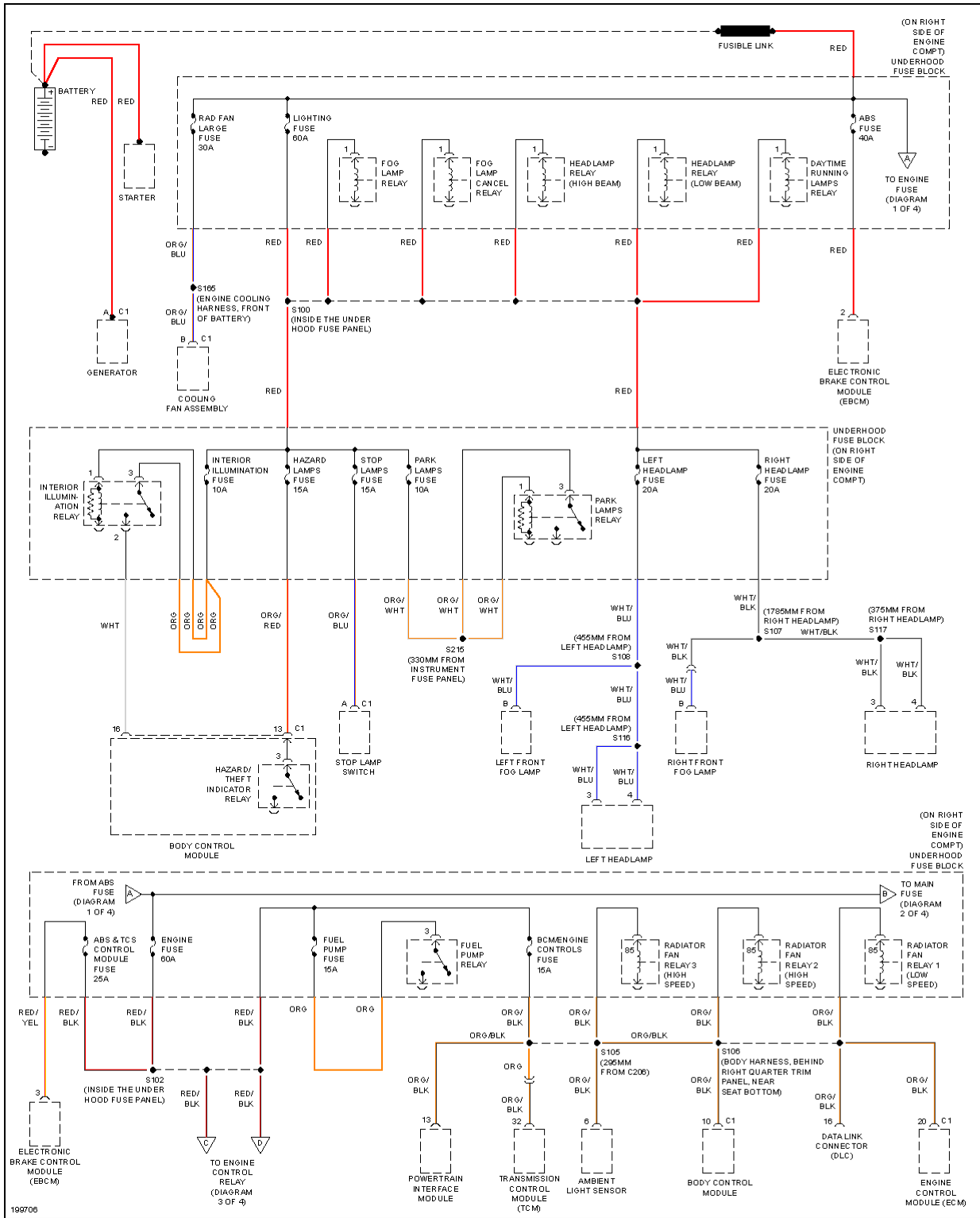
Fig. 29: Power Distribution Circuit (1 of 4)
