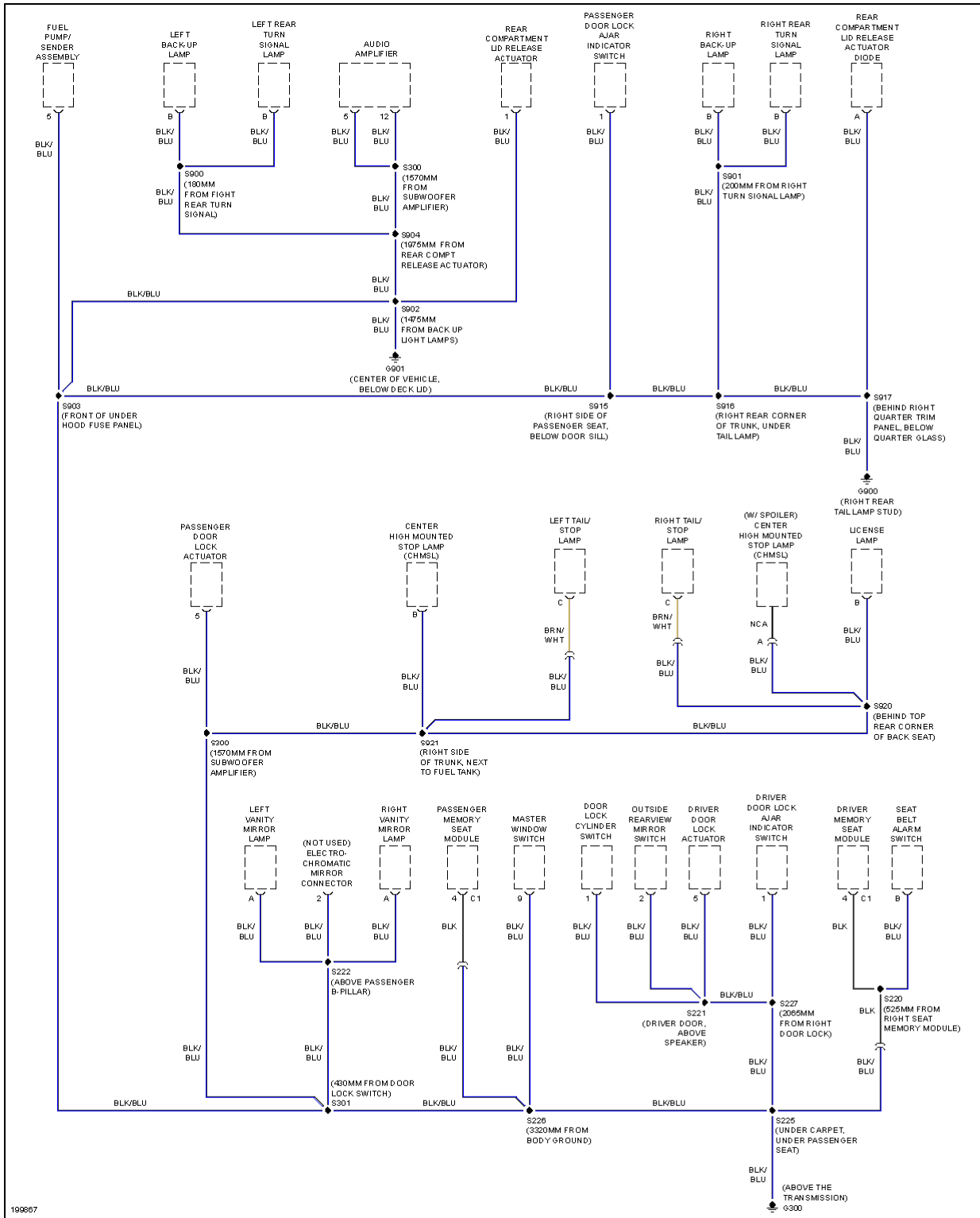
Fig. 22: Ground Distribution Circuit (3 of 3)
