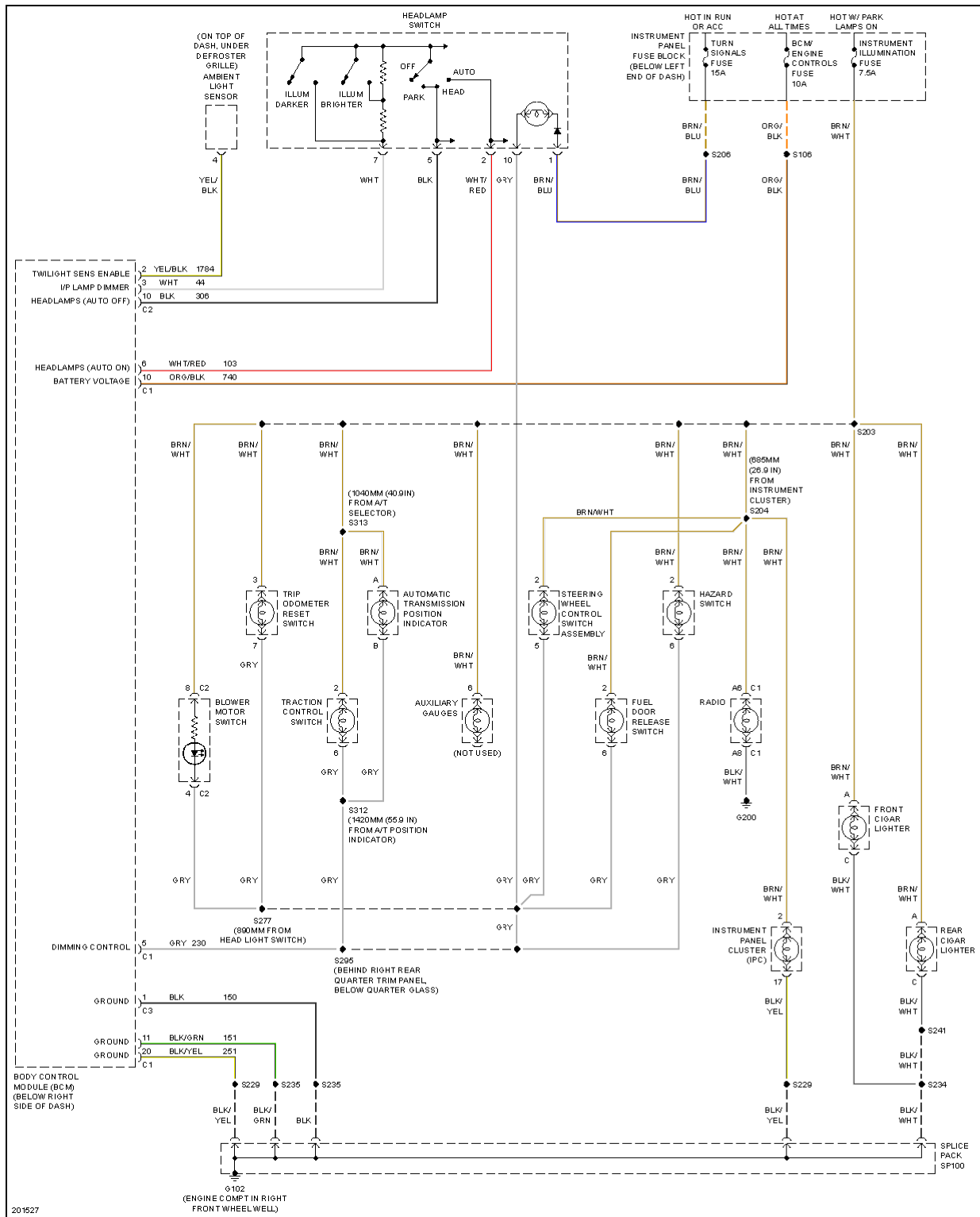
Fig. 28: Instrument Illumination Circuit
