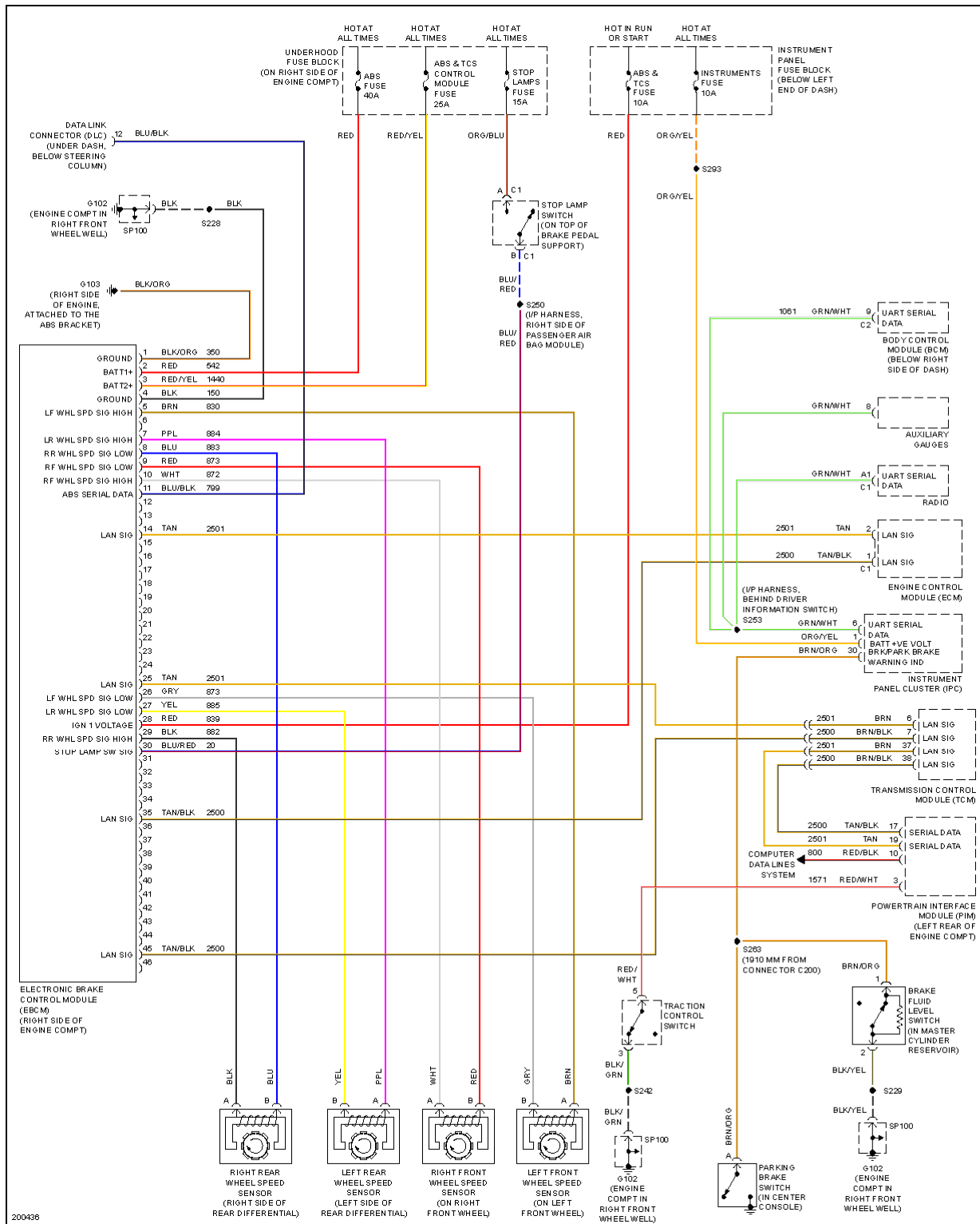
Fig. 4: Anti-lock Brakes Circuit
