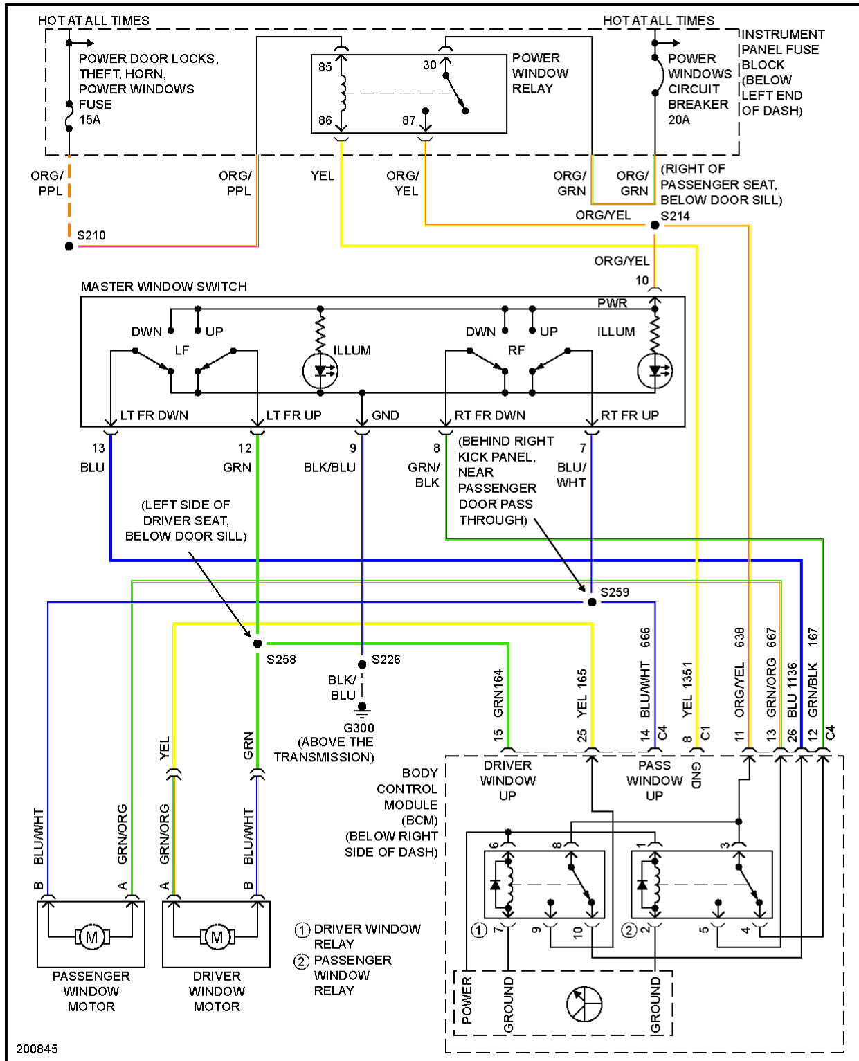
Fig. 36: Power Windows Circuit
