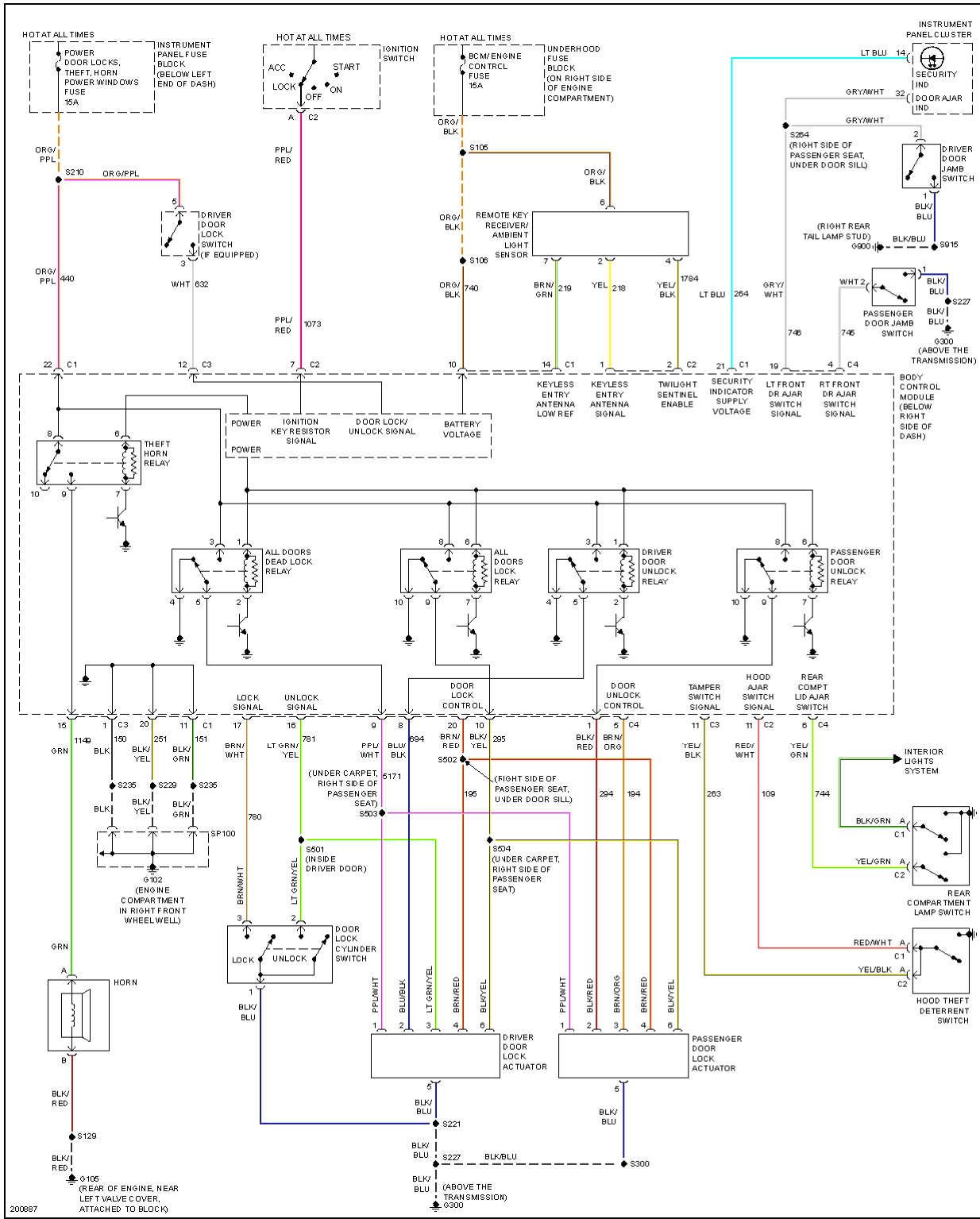
Fig. 5: Anti-theft Circuit
