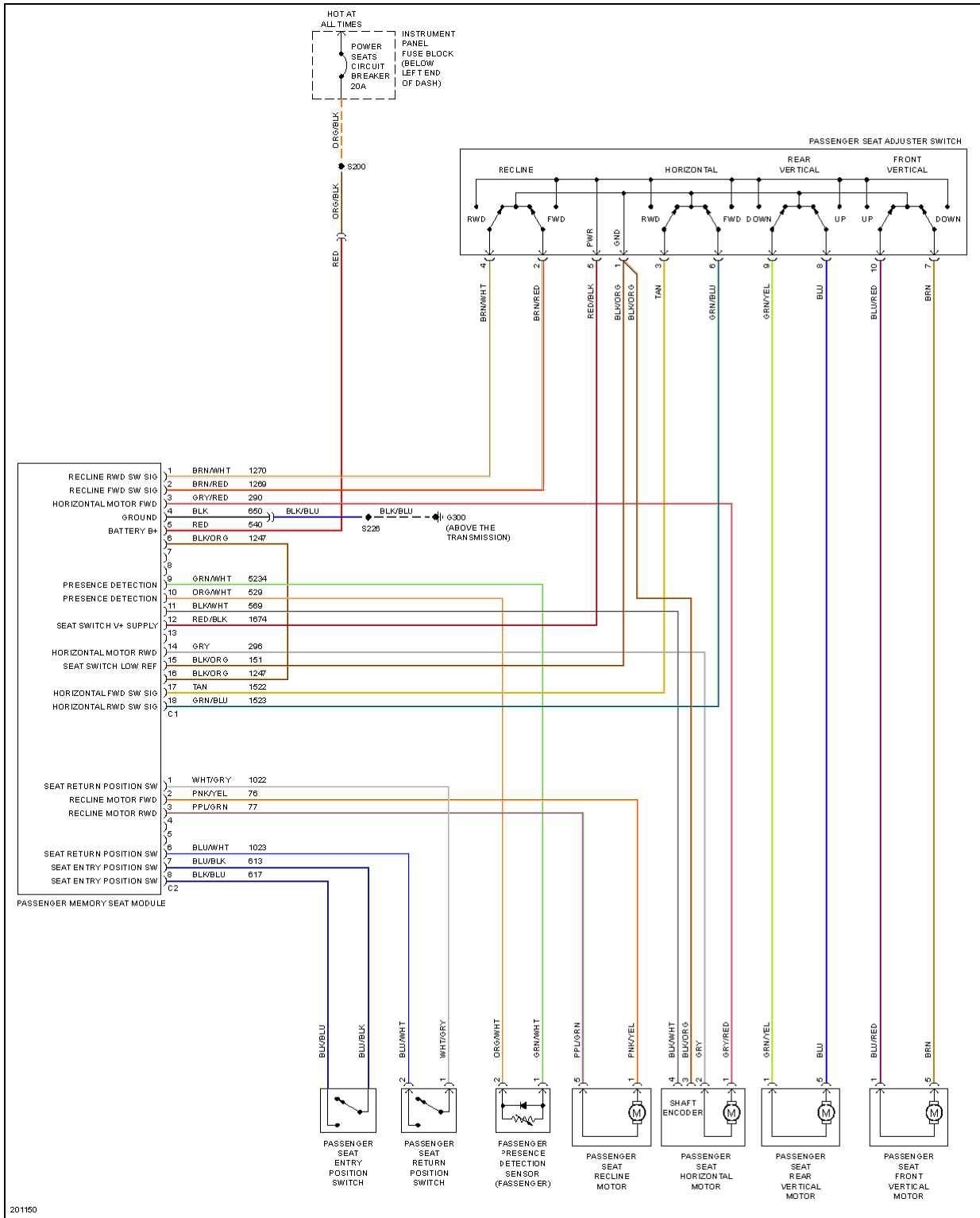
Fig. 35: Passenger Power Seat Circuit
