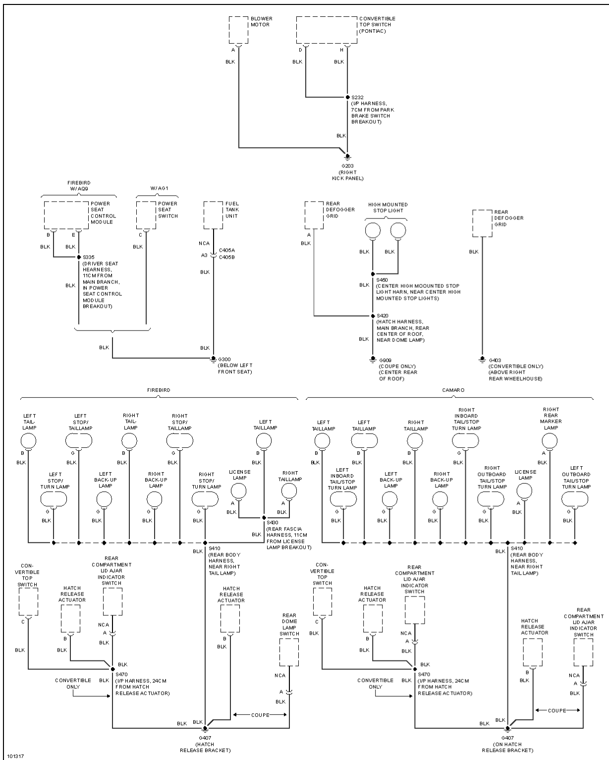
Fig. 23: Ground Distribution Circuit (3 of 3)
