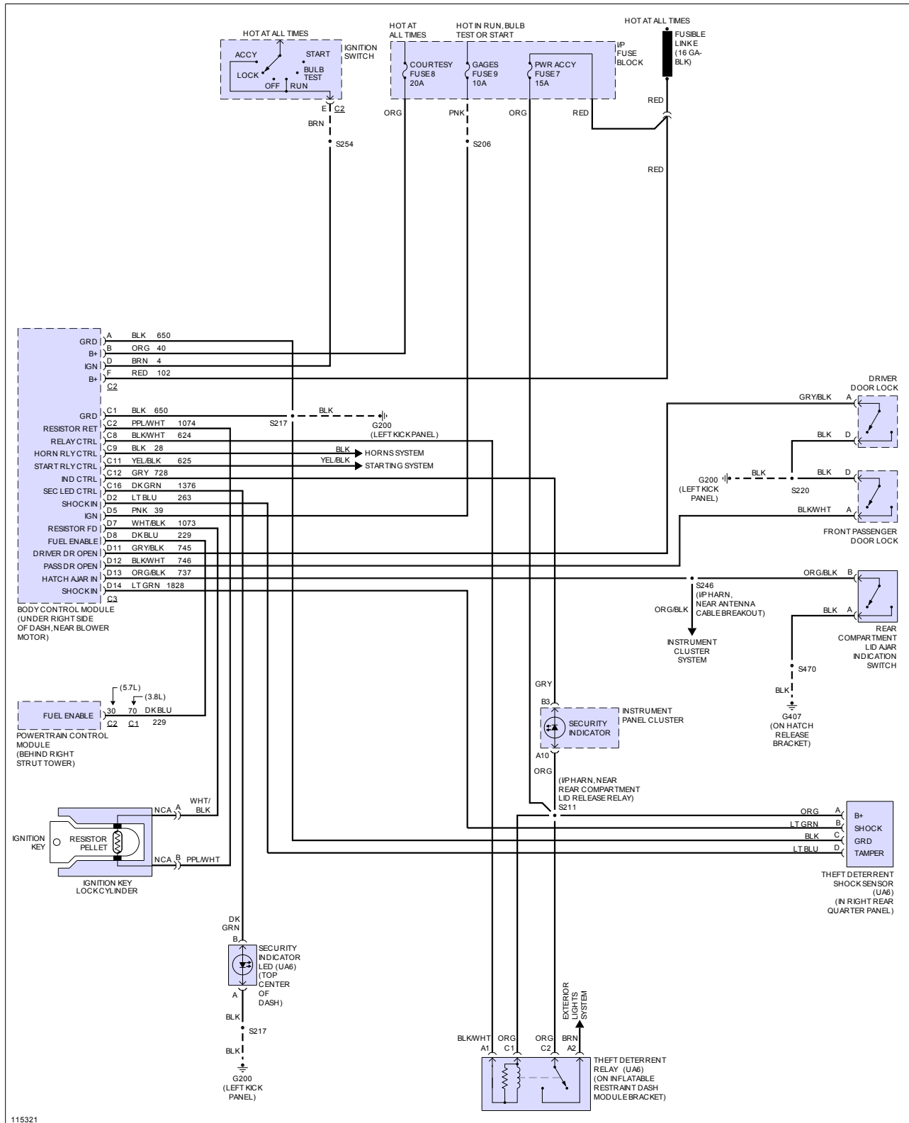
Fig 1: Anti-theft Circuit
